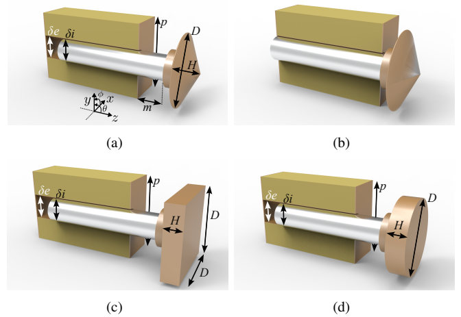
Fig. 1. 3-D views of mechanically RIS unit cells. (a) Proposed unit cell with cone-shaped end in state “0”, (b) unit cell with cone-shaped end and in state “1”, (c) unit cell with cube-shaped end and, (d) unit cell with cylinder-shaped end. The dimensions (in mm) are: D = 8.04 mm, H = 1.95 mm, p = 9 mm, \delta_e = 3 mm and \delta_i = 2.9 mm.
