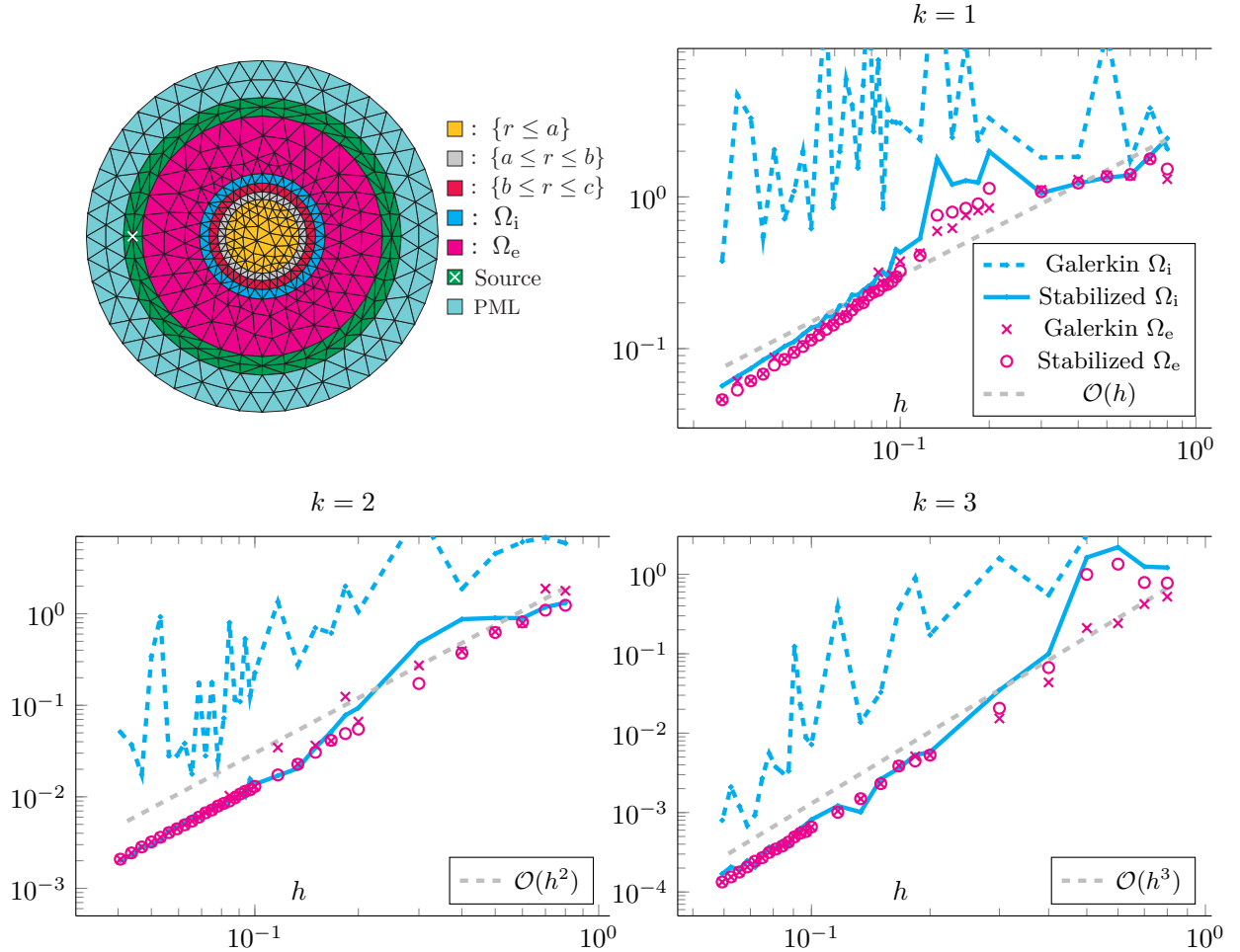
FIGURE 5. Upper left panel: computational setup. Other panels: Relative H^1 -error in \Omega_i and \Omega_e with respect to the reference solution (4.3) as a function of the mesh size. Here, h refers to an upper bound on the mesh size in \{r < a\} \cup \{r > c\} . The mesh size within the metamaterial \{a \leq r \leq c\} is bounded from above by h/3 .
