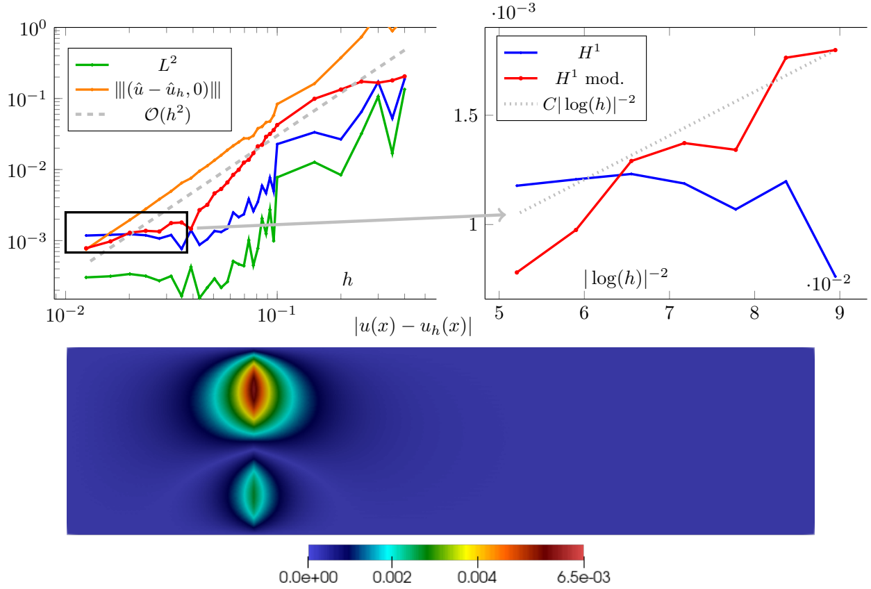
FIGURE 7. Results for the non-symmetric cavity with contrast inside the critical interval obtained with the stabilized method using k = 2 . The red line displays the error in the H^1 -norm obtained with a modified method for which we added the additional stabilization discussed in Remark 2.4. All other graphs display the results obtained with the original method. Notice that the x -axis in the right plot is given in terms of |\log(h)|^{-2} and that the error for the modified method looks almost like a straight line in this plot. The figure on the bottom displays the absolute error for the modified method on a mesh of size h \approx 0.028 .
