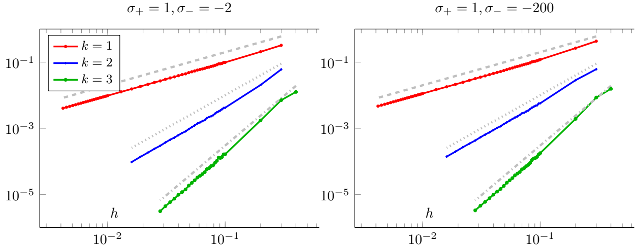
FIGURE 2. Relative error \|u - u_h\|_{H^1(\Omega_+ \cup \Omega_-)} / \|u\|_{H^1(\Omega_+ \cup \Omega_-)} for the symmetric cavity in the well-posed case on unstructured meshes.
