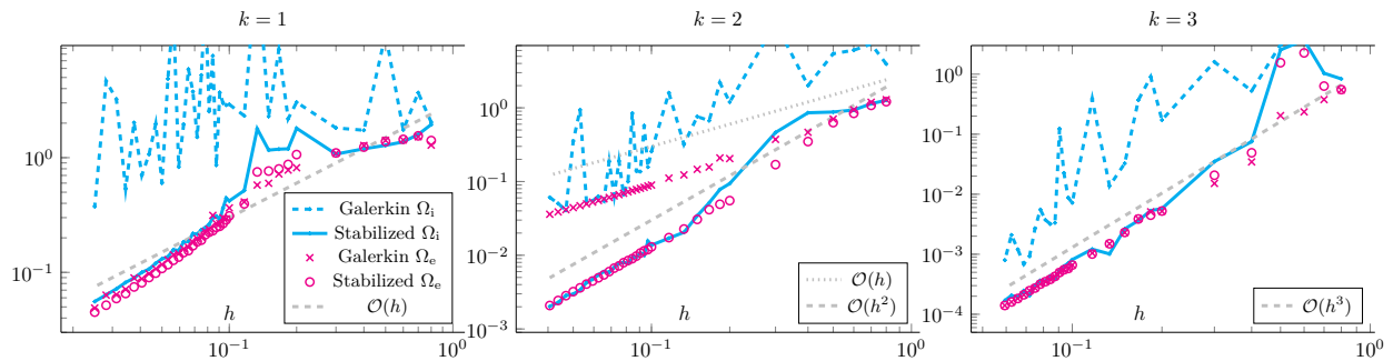
FIGURE 6. Relative H^1 -error in \Omega_i and \Omega_e with respect to the reference solution (4.3) when the parameter m in the PML profile (4.4) is chosen as m = 0 .
