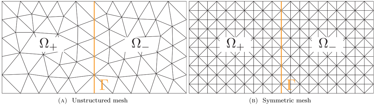
FIGURE 1. Meshes for the cavity problem.
