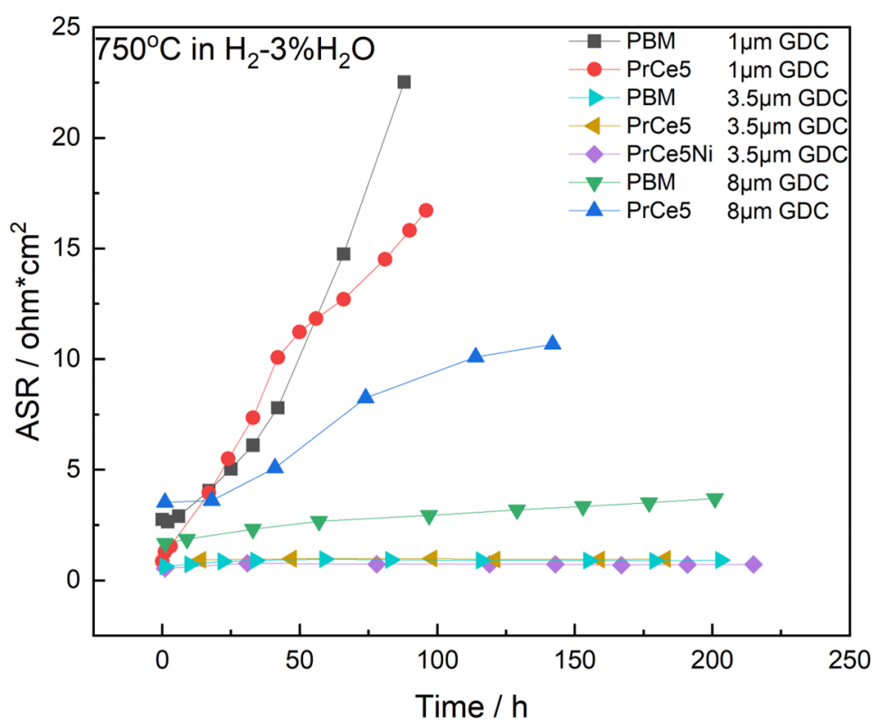
Figure 8. Impact of GDC buffer layer thickness on ASR performance over time for PBM, PrCe5 and PrCe5Ni anodes.
