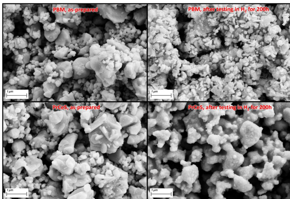
Figure 6. SEM images of the PBM and PrCe5 electrodes surfaces (a) before and (b) after hydrogen testing for 200 h revealing morphological changes.
