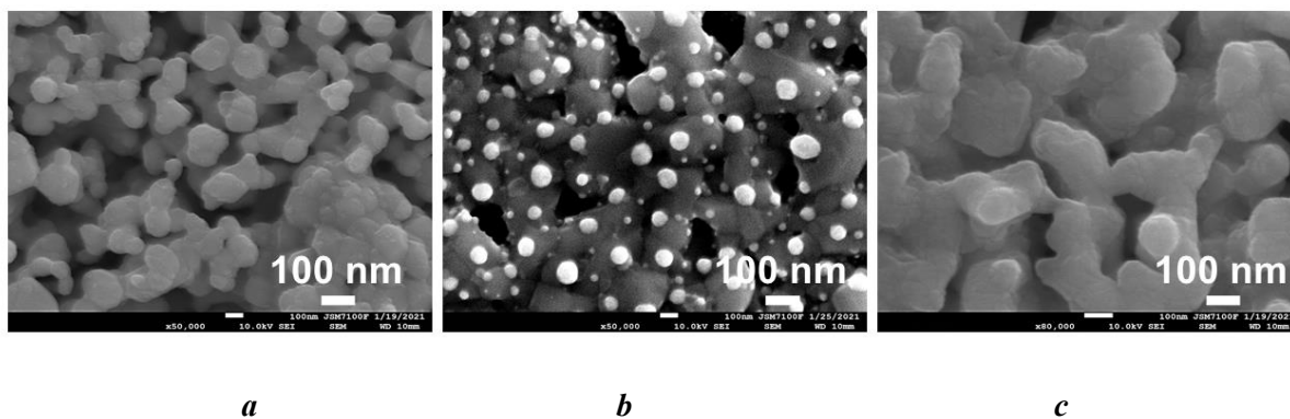
Figure 2. SEM images of (a) as prepared, (b) reduced where the exsolved Ni particles appear as white spheres, and (c) oxidized PrCe 5 Ni samples.
