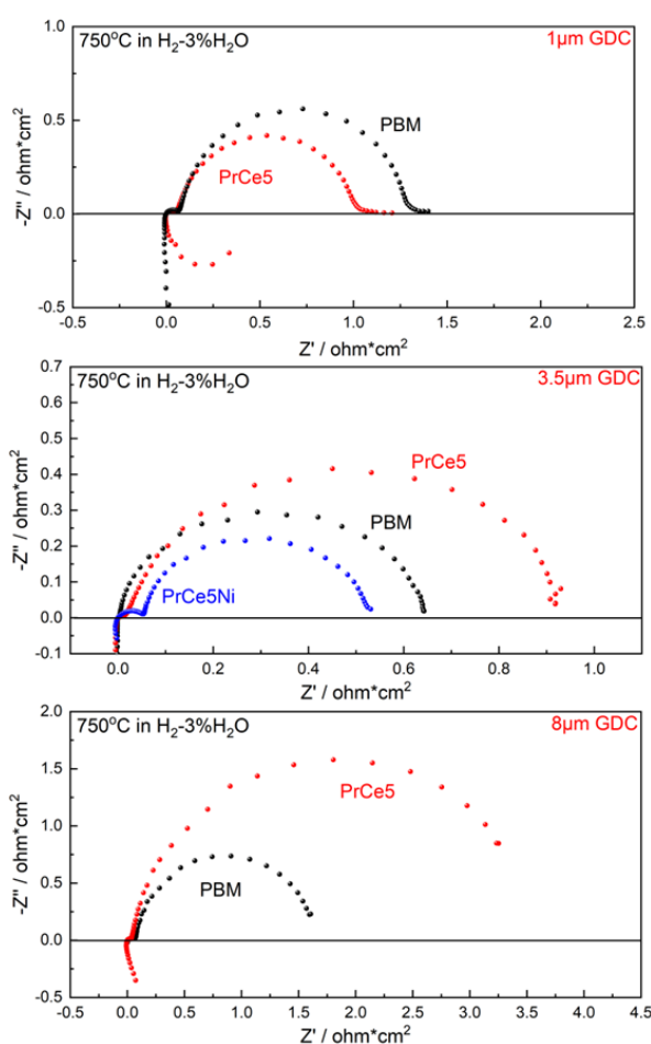
Figure 5. Nyquist plots for electrodes on GDC buffer layer with different thicknesses.
