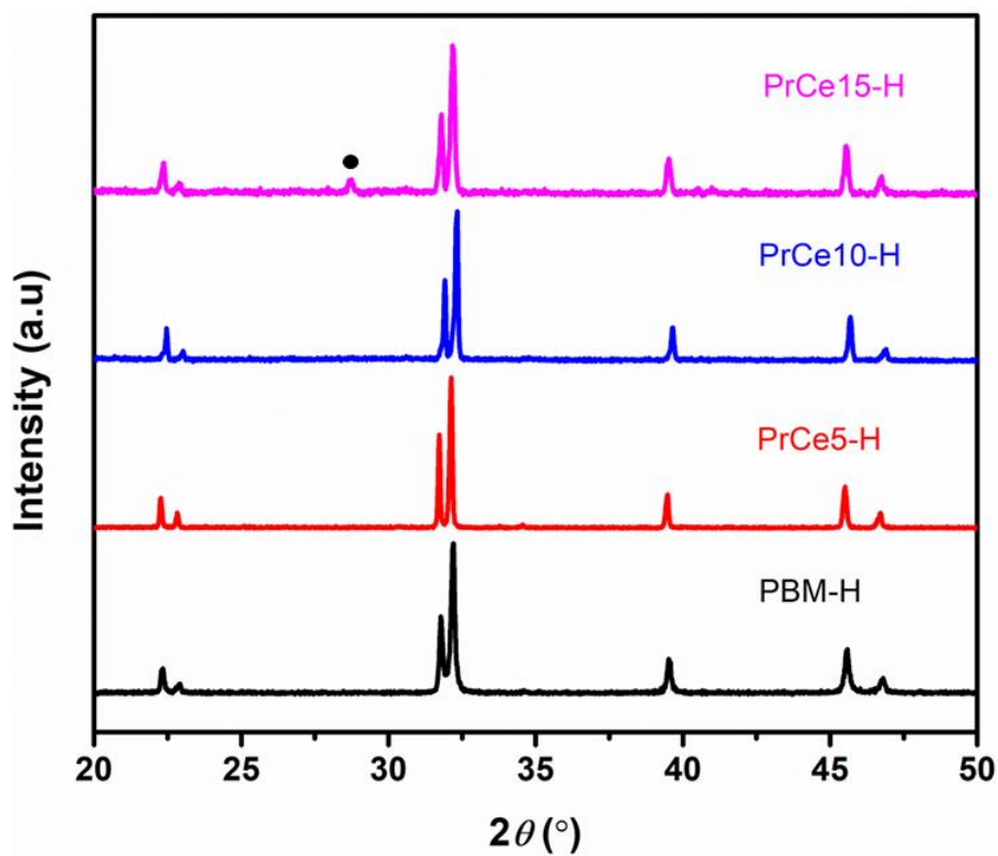
Figure 1. XRD patterns of as-prepared layered double perovskites. The peak from \text{CeO}_2 (●) in PrCe15-H is highlighted.
