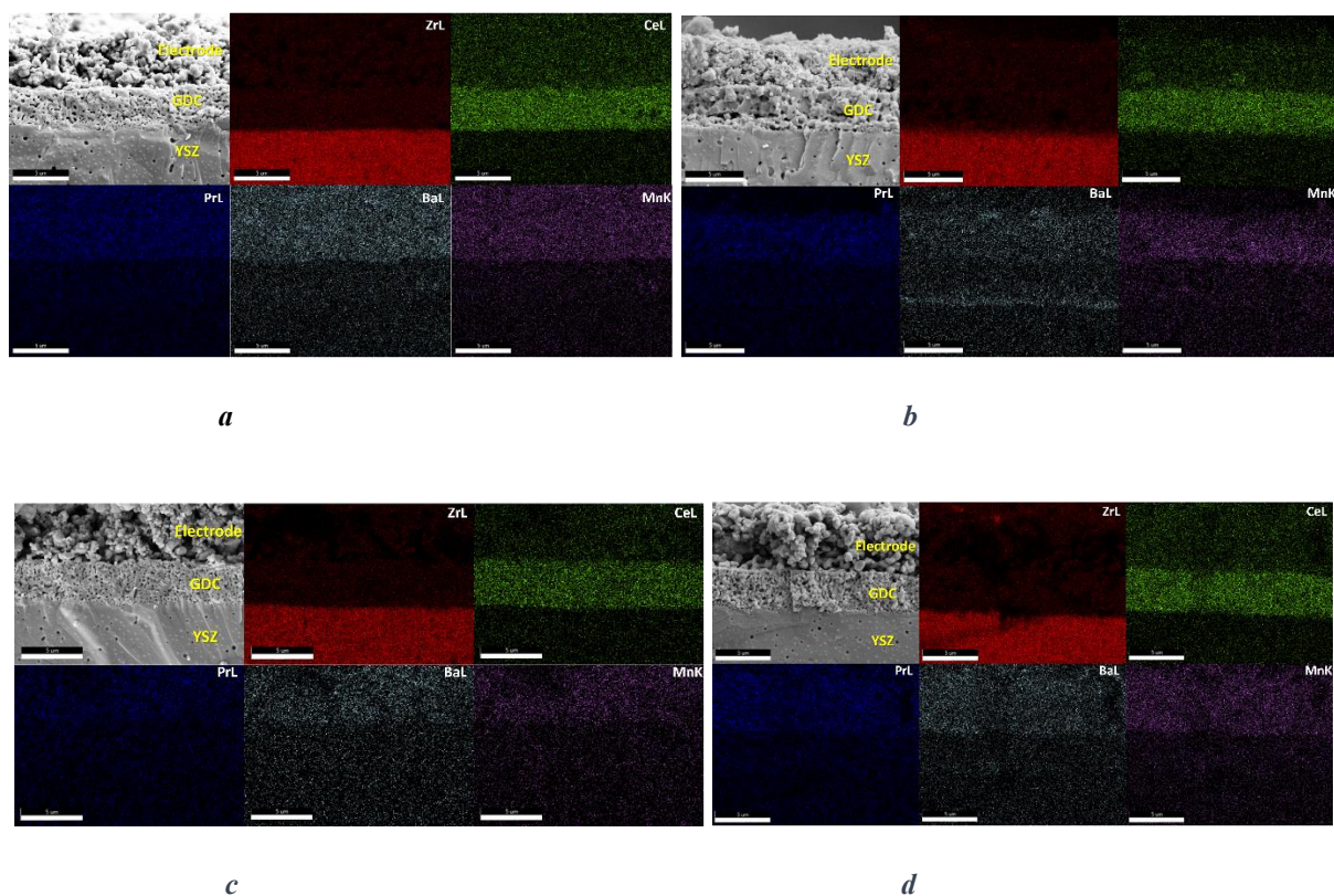
Figure 7. Comparison between (upper panels) PBM and (lower panels) PrCe5 electrodes. Panels (a) and (c) illustrate the baseline structure before testing, while panels (b) and (d) reveal changes after 200 h of H 2 exposure. Notably, the PBM electrode demonstrates significant barium diffusion through the GDC layer, in stark contrast to the PrCe5 electrode, where cerium doping effectively maintains structural integrity.
