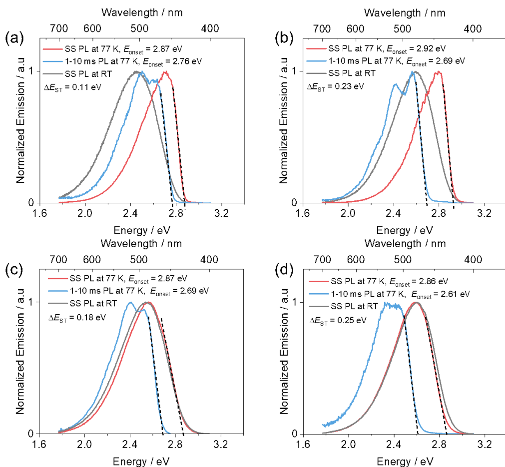
Figure 5. Steady-state PL at RT and 77 K and time-gated emission (1-10 ms) spectra at 77 K. a) (1,4)-tBuCzpPhTrz in 2-MeTHF glass ( \lambda_{\text{exc}} = 375 nm). b) (1,7)-tBuCzpPhTrz in 2-MeTHF glass ( \lambda_{\text{exc}} = 375 nm). c) (1,4)-tBuCzpPhTrz as a 10 wt% doped films in DPEPO ( \lambda_{\text{exc}} = 375 nm). d) (1,7)-tBuCzpPhTrz as a 10 wt% doped films in DPEPO ( \lambda_{\text{exc}} = 365 nm).
