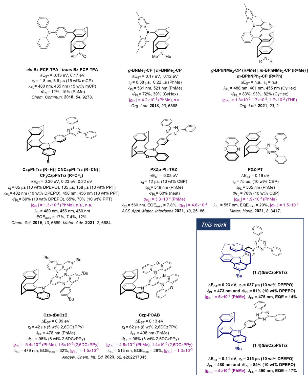
Figure 1. Summary of reported [2.2]paracyclophane-based TADF Emitters.
