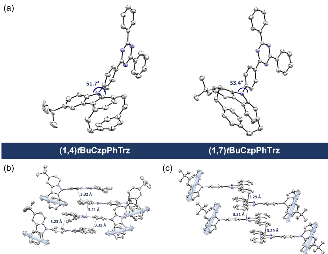
Figure 2. a) Molecular structures of (1,4) t BuCzpPhTrz (CCDC 2305740) and (1,7) t BuCzpPhTrz (CCDC 2261384). Displacement parameters are drawn at 50% probability level, hydrogens are omitted for clarity. Schematic presentation of the \pi - \pi stacking along the triazine planes in b) (1,4) t BuCzpPhTrz and c) (1,7) t BuCzpPhTrz .
