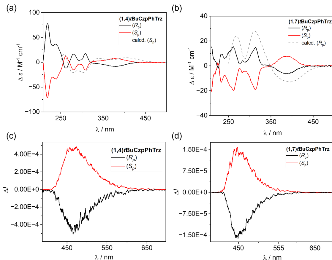
Figure 7. Experimental and calculated ECD spectra of a) ( R_p )/( S_p )-(1,4)- t BuCzpPhTrz and b) ( R_p )/( S_p )-(1,7)- t BuCzpPhTrz measured in tetrahydrofuran. Predicted spectra were calculated at the TD-DFT-M06/6-311++G(d,p) with an implicit tetrahydrofuran solvent field (cpcm). CPL spectra of c) ( R_p )/( S_p )-(1,4)- t BuCzpPhTrz and d) ( R_p )/( S_p )-(1,7)- t BuCzpPhTrz in toluene ( \lambda_{exc} = 350 nm).
