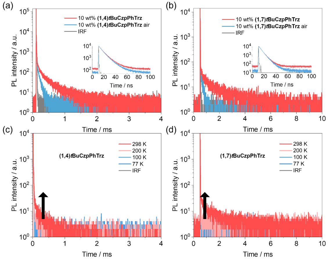
Figure 6. Time-resolved PL decay within millisecond and 100 ns time windows (inset) of 10 wt% doped films in DPEPO in air and under vacuum of a) (1,4)tBuCzpPhTrz ( \lambda_{\text{exc}} = 375 nm) and b) (1,7)tBuCzpPhTrz ( \lambda_{\text{exc}} = 375 nm). Temperature-dependent time-resolved PL decays of 10 wt% doped films in DPEPO of c) (1,4)tBuCzpPhTrz ( \lambda_{\text{exc}} = 375 nm) and d) (1,7)tBuCzpPhTrz ( \lambda_{\text{exc}} = 375 nm). IRF = instrument response function.
