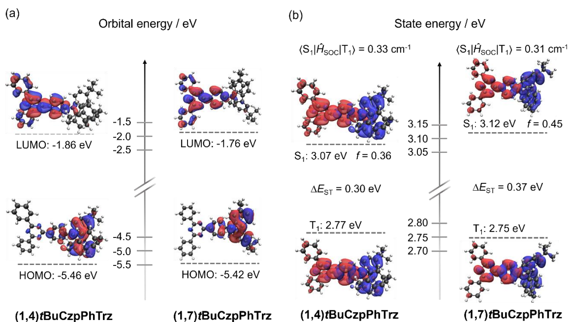
Figure 3. Theoretical modeling of a) the energies and electron density distributions of the HOMO/LUMO (ISO value = 0.02) and b) NTOs (particle and hole are represented by red and blue colors, respectively) and their associated vertical excitation energies of S_1 and T_1 states of (1,4)-tBuCzpPhTrz and (1,7)-tBuCzpPhTrz computed based on the ground-state optimized geometries, f is the oscillator strength.
