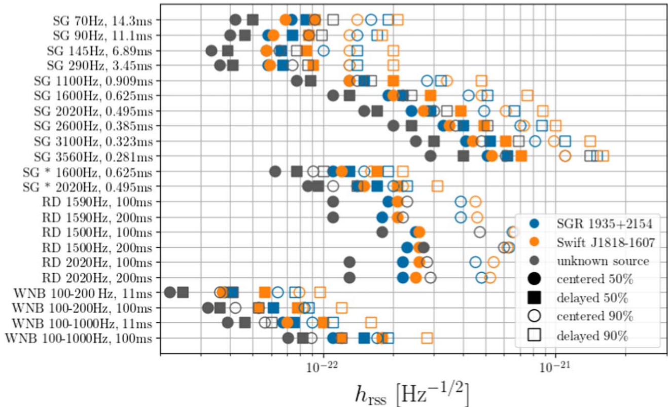
Figure 4. For each injection, we display the h_{\text{TSS}}^{50\%} and h_{\text{TSS}}^{90\%} values as measured by the most sensitive burst from each source in the short-duration search. The h_{\text{TSS}}^{50\%} values are marked by filled-in shapes, and the h_{\text{TSS}}^{90\%} values are not filled in. The vertical axis notes the waveform, where “SG” means sine-Gaussian and “RD” means ringdown. The frequency and duration of each injection are given as well. All of the sine-Gaussian and ringdown waveforms are elliptically polarized except for the ones denoted by “*,” which are circularly polarized. The numerical values of h_{\text{TSS}}^{50\%} can be found in Tables 6–8, while the numerical values of h_{\text{TSS}}^{90\%} can be found in Tables 9–11.
