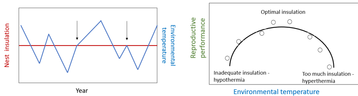
Figure 2. A. Hypothetical indication of a constant nest insulation over many years (red line on left panel) with the blue line indicating the environmental temperature. Nest insulation only matches the environmental temperature in certain years (arrows). B. the right panel shows the reproductive performance of the birds building the nests with optimal conditions producing the highest reproductive performance at some environmental temperatures. For cool temperatures the nest insulation is sub-optimal and reproductive performance is reduced. At high temperatures there is too much insulation and reproductive performance also suffers.
