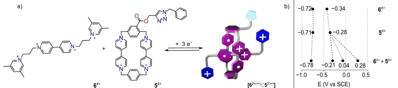
Figure 3. a) Reaction scheme to obtain [\text{6}^{2(+\bullet)}\text{C}5^{2(+\bullet)}] upon reduction and self-assembly. b) Genetic diagram displaying the redox processes observed in the DPV of 5^{4+} , 6^{4+} , and a 1 mM mixture of both. Conditions: ACN, \text{TBAPF}_6 100 mM. All positive charges are balanced by \text{PF}_6^- counterions, which are omitted for clarity.
