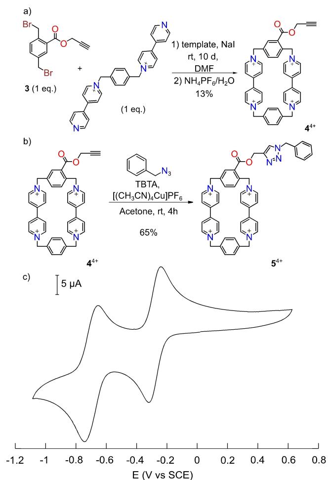
Figure 2. a) Reaction scheme for the synthesis of a) 4 4+ and b) 5 4+ . TBTA: tris(benzyltriazolylmethyl)amine. All positive charges are balanced by PF 6 - counterions, which are omitted for clarity. c) CV of 5 4+ at 200 mV s -1 scan rate. Conditions: ACN, TEAPF 6 100 mM.
