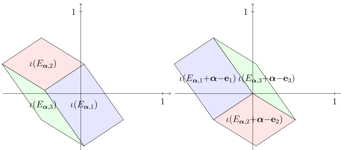
FIGURE 4. The ( \iota -representation of the) parallelepipeds E_{\boldsymbol{\alpha},i} and their \tilde{T}_{\boldsymbol{\alpha}} -images for d = 3 , \boldsymbol{\alpha} = (0.48, 0.32, 0.2) .
