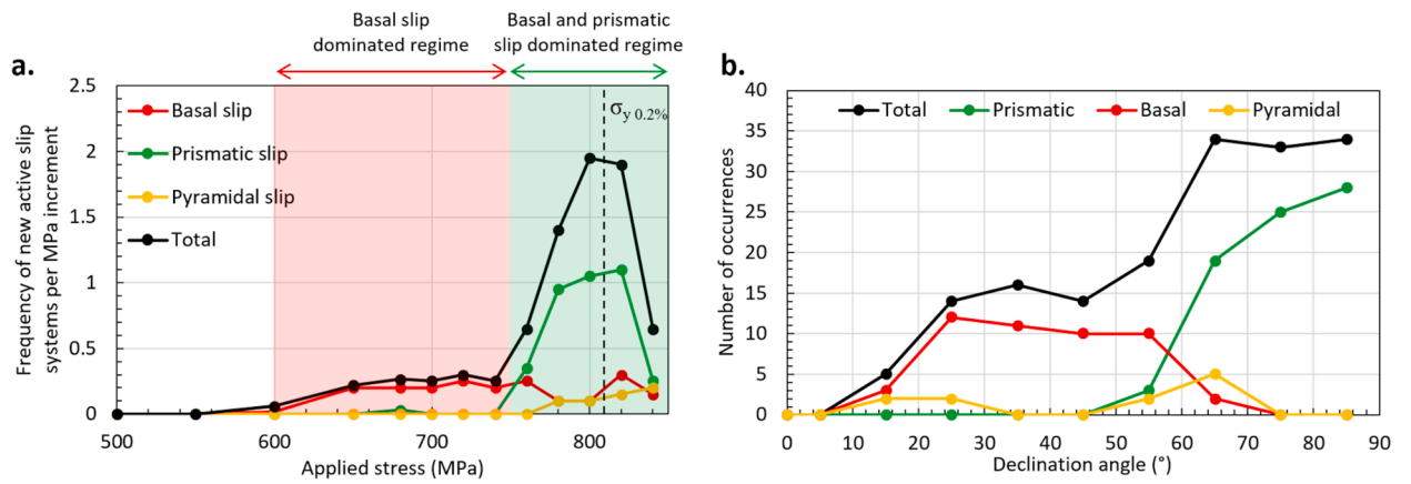
Fig. 6. a. Basal, prismatic and pyramidal slip activation as a function of the applied stress, b. Distribution of basal, prismatic and pyramidal slip with respect to the misorientation between the c-axis of the HCP lattice and the loading direction.
