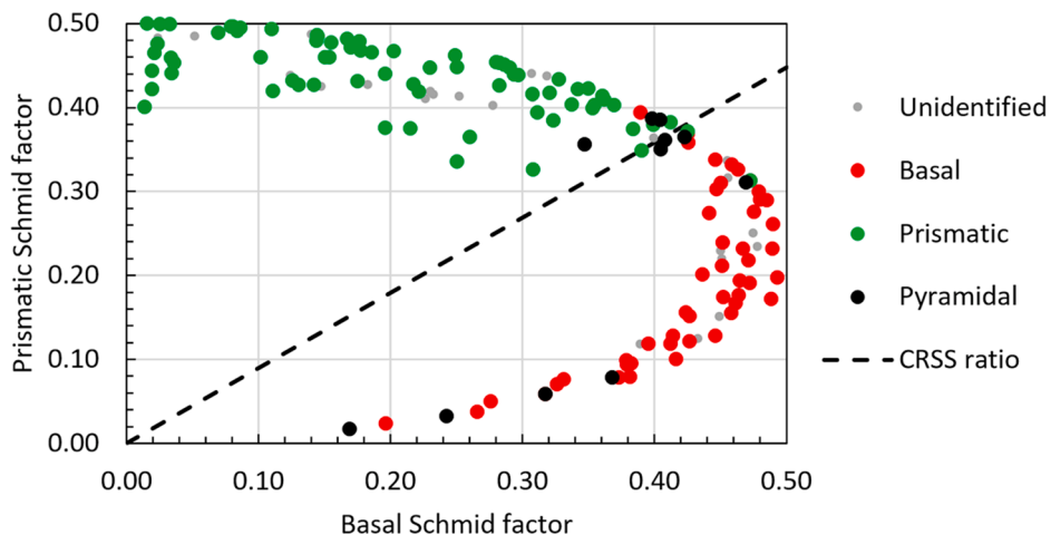
Fig. 7. Analyzed slip traces plotted with respect to the basal and prismatic Schmid factors at the end of the in situ test, suggesting very similar CRSS values for both slip modes but a slightly higher value for basal slip. The presently determined ratio of basal to prismatic CRSS values reveal a good agreement with experimental data.
