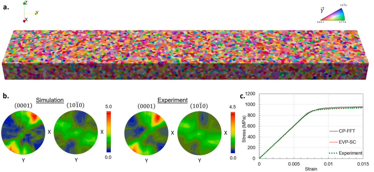
Fig. 16. a. 3D view of the polycrystalline aggregate generated using Dream3D, b. Comparison of texture in the experiment and in the simulation, and c. Comparison of macroscopic stress – strain curves obtained from experiments and different simulation techniques.
