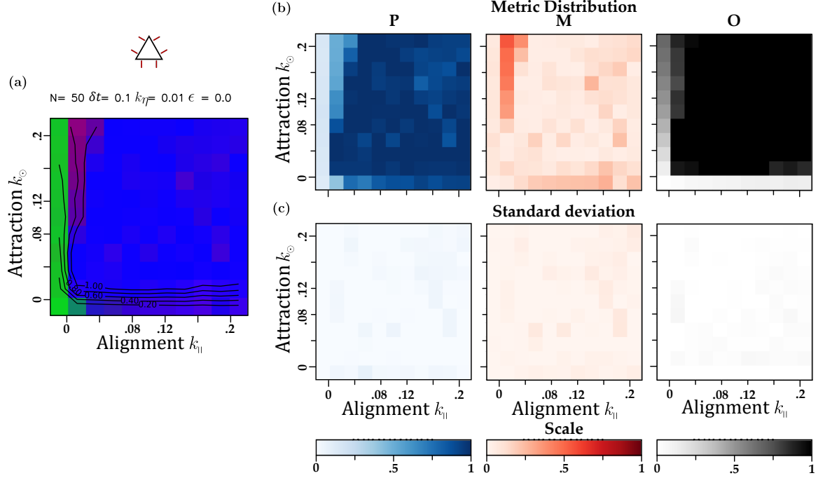
Fig. S 17. Phase diagram for the Omniscient model of a flock size of 50 individuals, k_\eta = 0.01 and no blind angle. a) Integrated metrics, b) Separated metrics and c) Variance between the 10 experiments final metrics.
