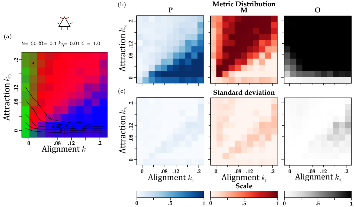
Fig. S 18. Phase diagram for the Omniscient model of a flock size of 50 individuals, k_\eta = 0.01 and maximum blind angle. a) Integrated metrics, b) Separated metrics and c) Variance between the 10 experiments final metrics.
