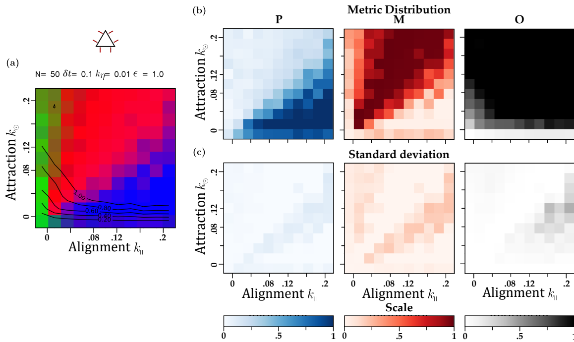
Fig. S 18. Phase diagram for the Omniscient model of a flock size of 50 individuals, k_\eta = 0.01 and maximum blind angle. a) Integrated metrics, b) Separated metrics and c) Variance between the 10 experiments final metrics.
