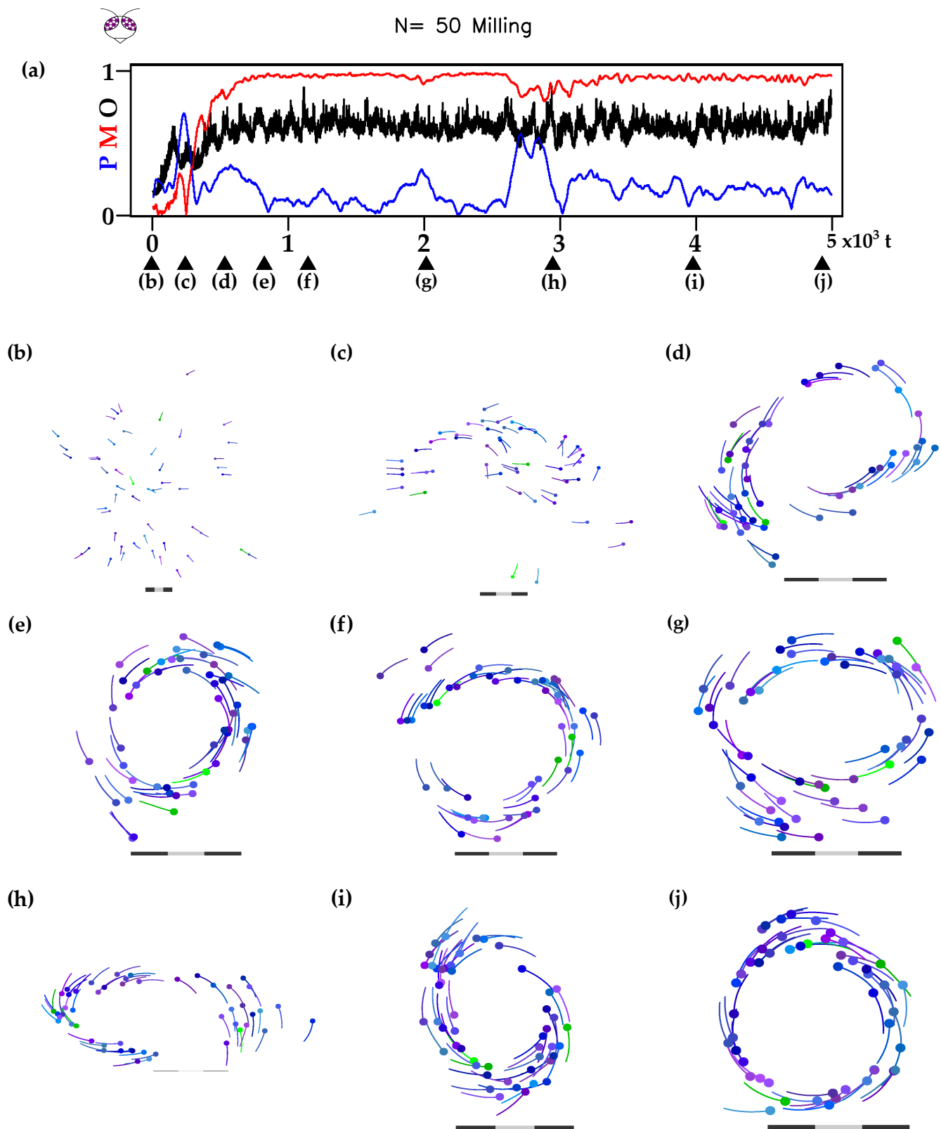
Fig. S 23. Snapshot of the time step stability at \delta t=0.1 for the Visual model. Reproduction of a milling phase for a flock size of 50 individuals, k_{\odot} = 0.06, k_{\parallel} = 0.06 and k_{\eta} = 0.01 . a) Evolution of the flock metrics, b-j different snapshots. , Video S3 ( https://youtu.be/1KMUSwcKyN8 ).
