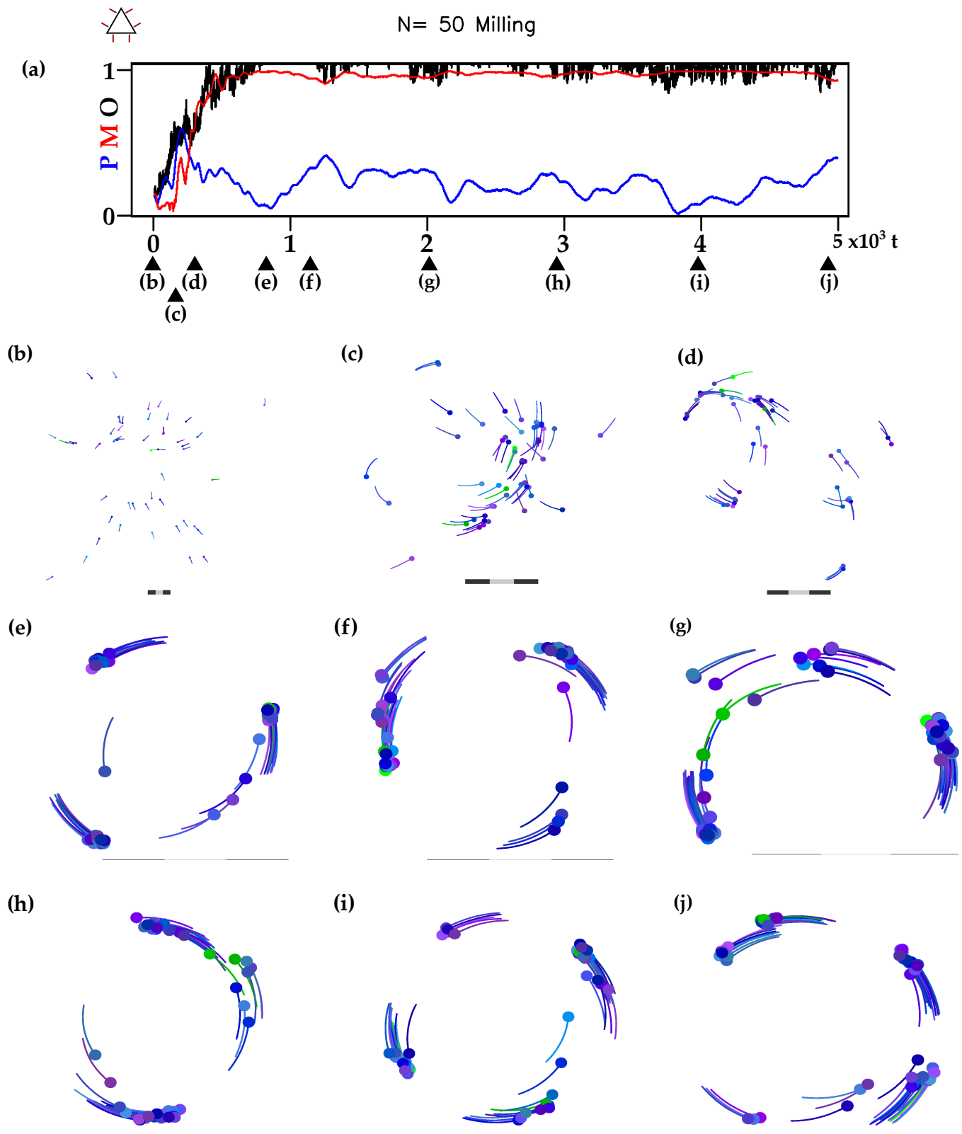
Fig. S 32. Milling phase reproduction for a flock size of 50 individuals for the Omniscient model. k_\eta = 0.06 k_\eta = 0.06 k_\eta = 0.01 and maximum blind angle , Video S12 ( https://youtu.be/CWpTSvr_zBk ).
