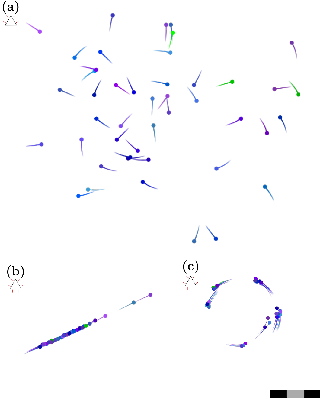
Fig. S 14. Illustration of the phases observed for the omniscient model and a flock size of N = 50 individuals. With k_{\eta} = 0.01 . The scale bar measures 30a ( 10a each section). We observe three phases: (a) Swarming ( k_{\odot} = 0.06 , k_{\parallel} = 0 , \epsilon = 0 ); (b) Schooling ( k_{\odot} = 0.06 , k_{\parallel} = 0.2 , \epsilon = 1 ); (c) Milling ( k_{\odot} = 0.06 , k_{\parallel} = 0.06 , \epsilon = 1 ).
