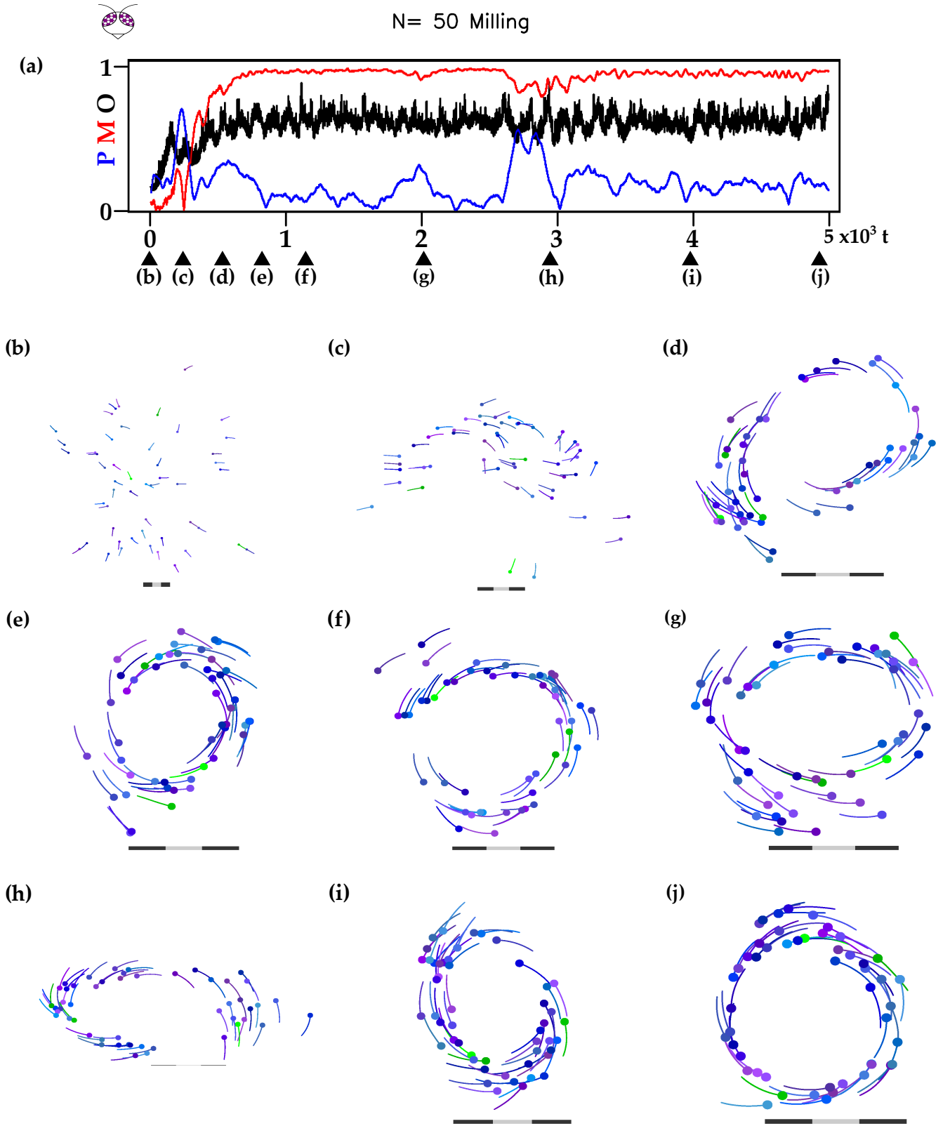
Fig. S 23. Snapshot of the time step stability at \delta t=0.1 for the Visual model. Reproduction of a milling phase for a flock size of 50 individuals, k_{\odot}=0.06, k_{\parallel}=0.06 and k_{\eta}=0.01 . a) Evolution of the flock metrics, b-j different snapshots. , Video S3 ( https://youtu.be/1KMUSWcKyN8 ).
