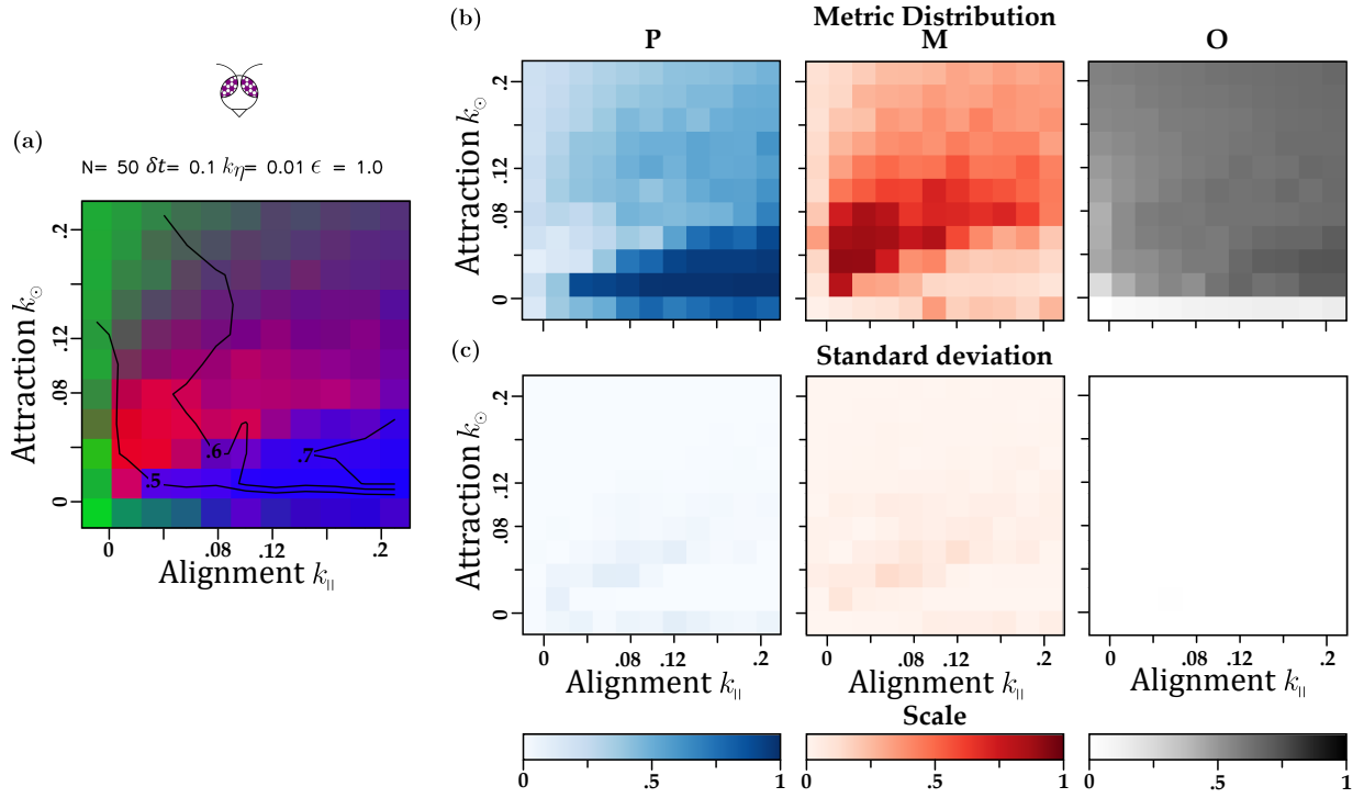
Fig. S 11. Phase diagram for the Visual model of a flock size of 50 individuals, k_\eta = 0.01 and maximum blind angle. a) Integrated metrics, b) Separated metrics and c) Variance between the 10 experiments final metrics.
