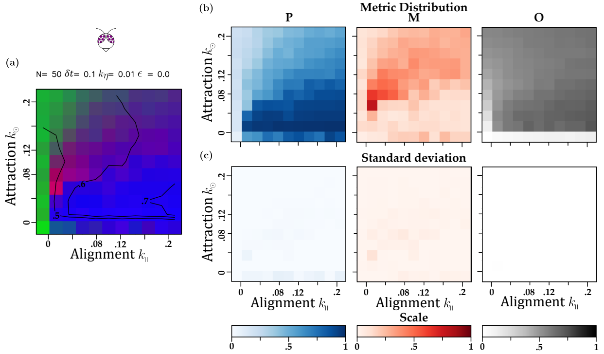
Fig. S 10. Phase diagram for the Visual model of a flock size of 50 individuals, k_\eta = 0.01 and no blind angle. a) Integrated metrics, b) Separated metrics and c) Variance between the 10 experiments final metrics.
