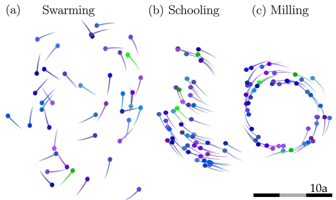
FIG. 2. Illustration of the phases observed for N = 50 individuals. The scale bar measures 30a in total ( 10a for each section). The parameters \epsilon = 1 and k_\eta = 0.01 are fixed. We observe three phases when varying the other two parameters: (a) swarming ( k_\odot = 0.1 , k_\parallel = 0 ); (b) schooling ( k_\odot = 0.06 , k_\parallel = 0.2 ); and (c) milling ( k_\odot = 0.1 , k_\parallel = 0.04 ).
