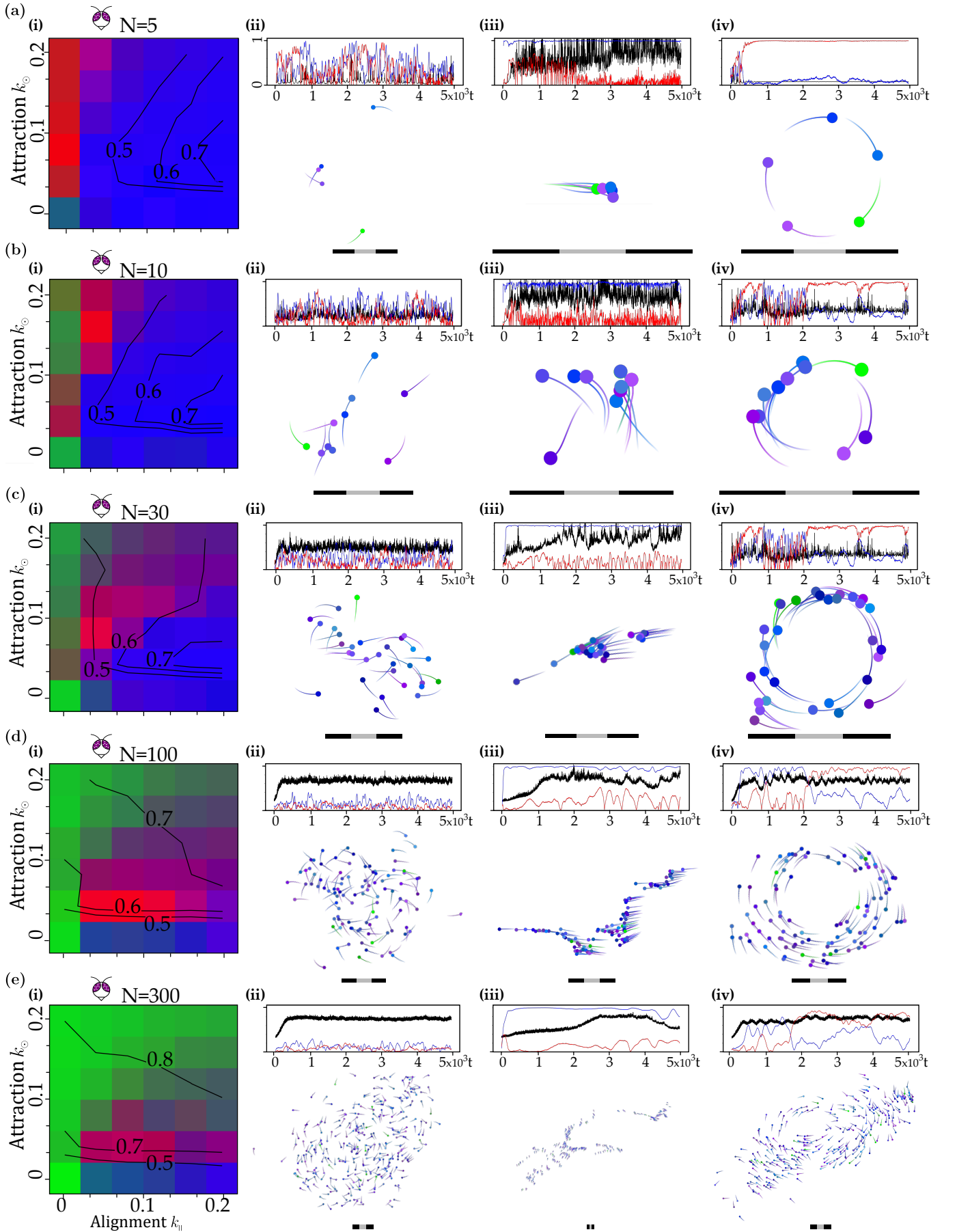
Fig. S 9. Phase Diagram and Phase Reproduction for different Flock sizes for the Visual model. i) Phase Diagram, ii)Swarming, iii)Schooling, iv)Milling. a) N=5 , b) N=10 , c) N=30 , d) N=100 , e) N=300 .
