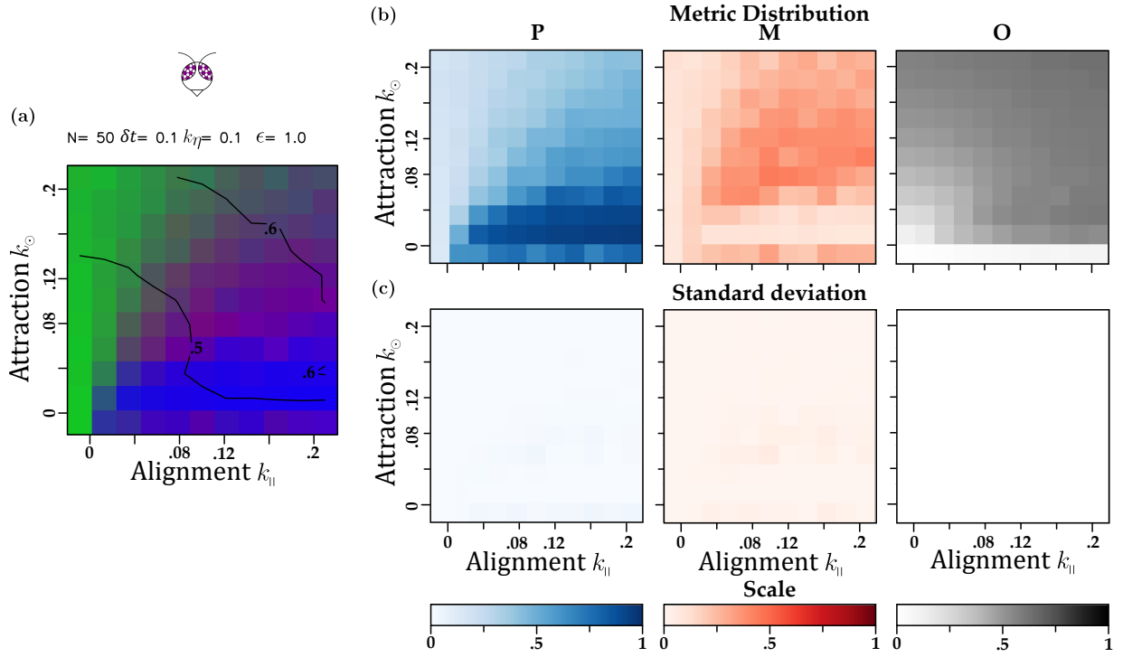
Fig. S 13. Phase diagram for the Visual model of a flock size of 50 individuals, k_\eta = 0.1 and maximum blind angle. a) Integrated metrics, b) Separated metrics and c) Variance between the 10 experiments final metrics.
