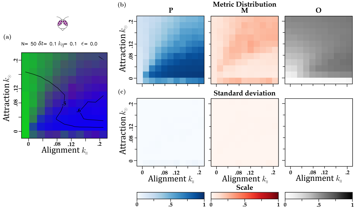
Fig. S 12. Phase diagram for the Visual model of a flock size of 50 individuals, k_\eta = 0.1 and no blind angle. a) Integrated metrics, b) Separated metrics and c) Variance between the 10 experiments final metrics.
