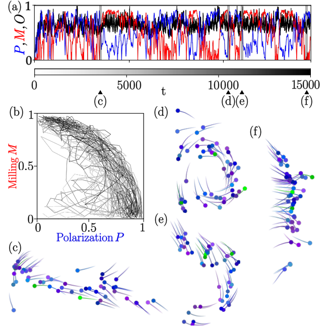
FIG. 4. Example of the bistability observed in the visual model (parameter values: \epsilon = 1 , k_\odot = 0.1 , k_\parallel = 0.2 , and k_\eta = 0.01 ). (a) Time series of the three metrics P , M , and O . (b) Trajectories of the collective behavior in the (M, P) -plane. Illustration of the phases: (c) schooling-milling transition; (d) milling; (e) milling-schooling transition; and (f) schooling.
