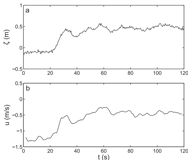
Figure 17. Tidal bore at the Garonne field site (Podensac), for a large spring tidal range at the estuary mouth ( Tr_0 = 5.1 m), and large river discharge ( Q_0 = 681 m 3 /s). Measurements from an ADCP current meter sampled at 2 Hz. TBG1 campaign, 2 March 2010. (a) Surface elevation \zeta ; (b) depth-integrated along-channel velocity u .
