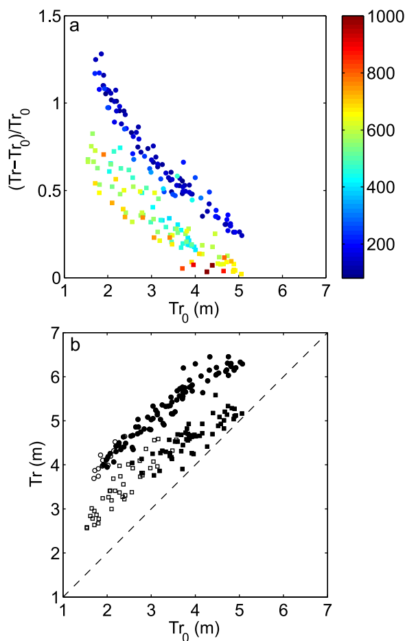
Figure 10. (a) tidal amplification ratio (Tr - Tr_0) / Tr_0 as a function of Tr_0 ; the colormap shows the freshwater discharge, Q_0 , in m^3/s . (b) tidal range at the Garonne field site, Tr , as a function of Tr_0 ; close and open symbols correspond to tidal wave regimes with and without tidal bore respectively. Square symbol, TBG1 campaign; circle symbol, TBG2 campaign.
