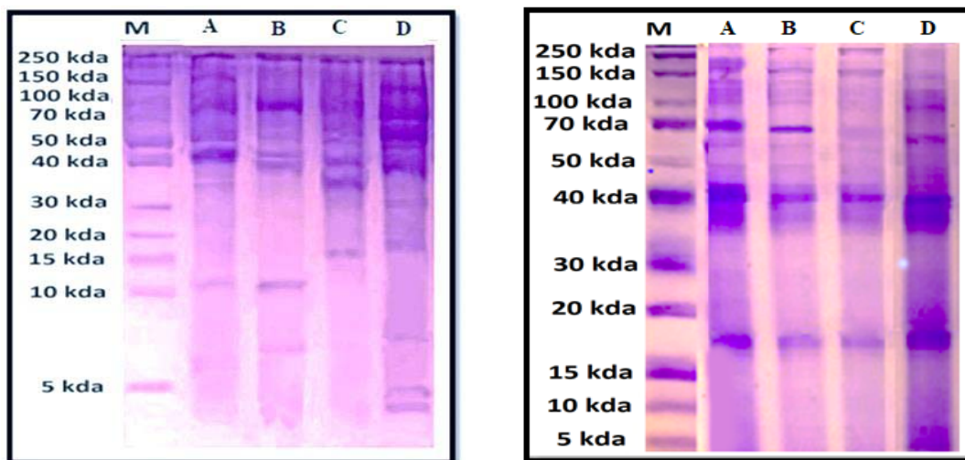
Figure 2. SDS-PAGE gel for honey bee hemolymph extracts dissolved in PBS (Figure 2A) or DMSO (Figure 2B) where, (A): Bee's hemolymph from a hive in Port Said, (B): from Ismailia governorate, (C): from Suez governorate, (D): from Saint Catherine. M: marker. The molecular weights of the proteins and their amounts are expressed by colour intensity of the protein bands.
