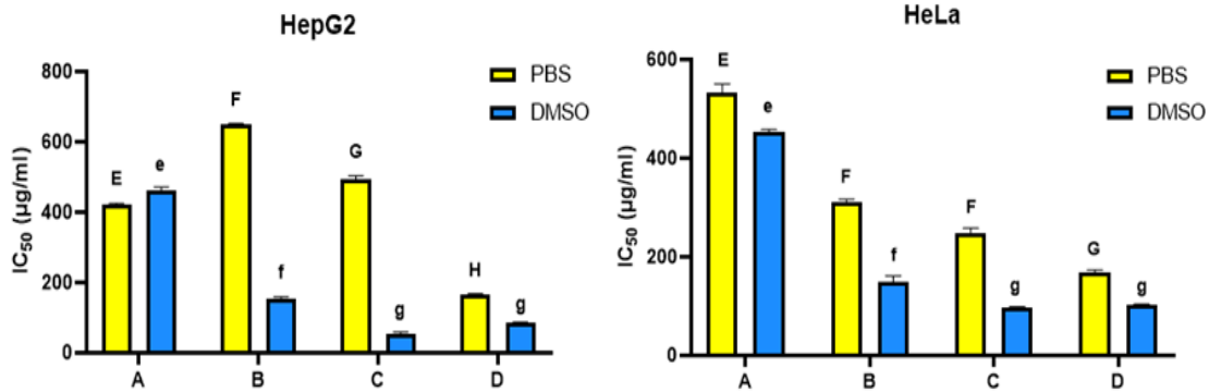
Figure 4. IC 50 in microgram/ml of hemolymph extracts of honey bees against Hepg2 and HeLa cell lines, in either solvents PBS or DMSO where, (A): Bee's hemolymph from a hive in Port Said, (B): from Ismailia governorate, (C): from Suez governorate, (D): from Saint Catherine. Bars and error bars represent the mean values \pm SE obtained from triplicate measurements. Different letters above bars indicate significant differences (Tukey's test, P < 0.05 ): uppercase letters show comparisons across PBS dissolved samples; lowercase letters show comparisons across DMSO dissolved samples.
