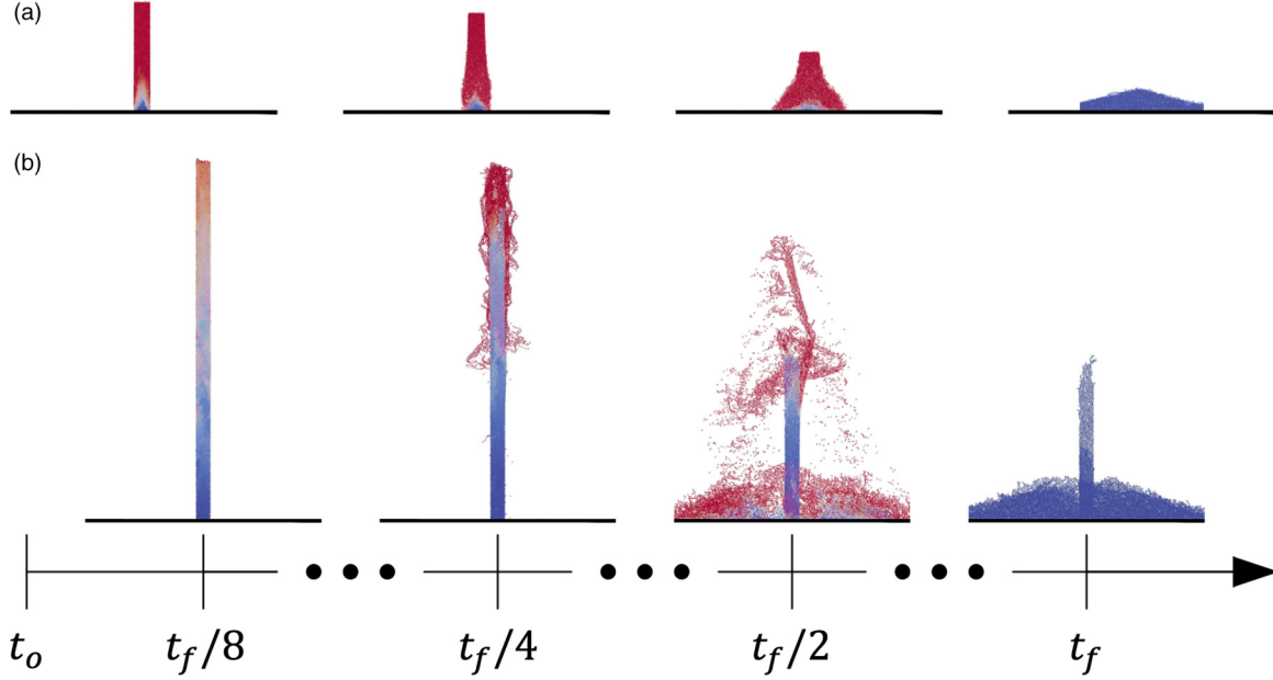
FIG. 10. Collapse sequence for a column with (a) N_a = 3 arms and an initial height H_0/D = 66 and (b) for N_a = 8 and H_0/D = 240 . t_f corresponds to the final time from which the heap is at rest. The color scale represents the particles' velocity.
