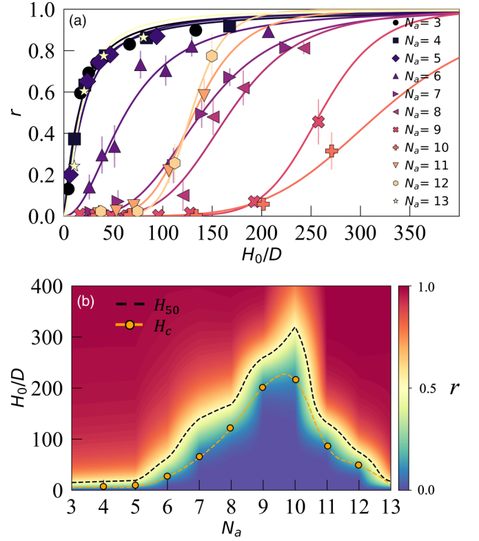
FIG. 5. (a) Evolution of the collapse ratio r of the columns as a function of the scaled initial height H_0/D , for columns composed of star-shaped particles with different numbers of arms N_a . Error bars represent the standard error between several repetitions for each H_0 . The lines show a fit of Eq. (3). (b) Stability phase diagram as a function of N_a and the scaled initial height H_0/D . The color scale is proportional to r . The evolution of the critical height H_c and the crossover height H_{50} (see text for a definition) is also shown using dashed lines.
