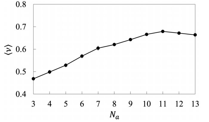
FIG. 7. Averaged packing fraction, \langle \nu \rangle , as a function of the number of arms N_a . Data points and bars (too small to be seen) represent the mean and standard error over all repetitions and for all column heights H_0 .
