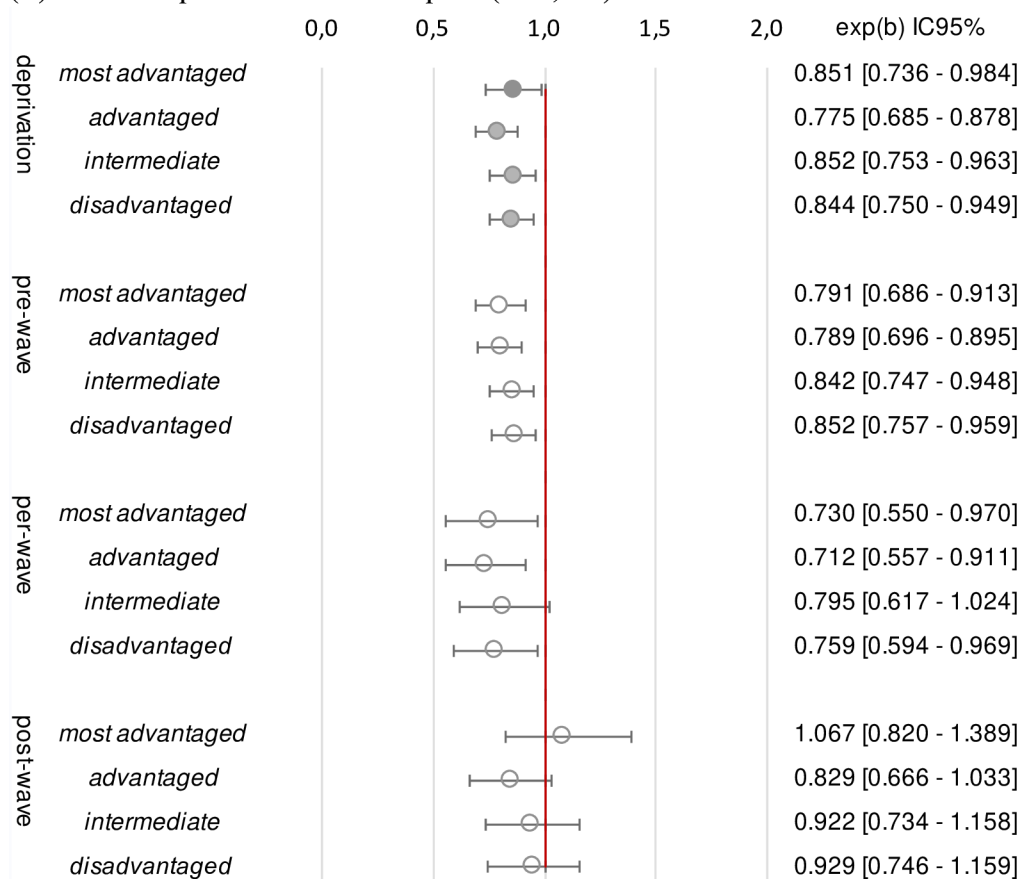
Figure 2 Estimation of each clinical and social factor (95% CI) on FMC-to-procedure time. Estimated overall effects expressed as \exp(\beta) with 95% CI; results of multivariate linear regression mixed models; variable to be explained: Y = \log(\text{FMC-to-procedure time}) ; (A) results adjusted on period and gender; (B) cardiovascular history was a history of stroke, transient ischaemic attack, coronary artery disease or myocardial infarction; results adjusted on period, age, gender, diabetes, hypertension, dyslipidaemia, obesity and smoking as risk factors; (C) the reference modality for the deprivation index Fdep15 in five categories was 'most disadvantaged'; results adjusted on period, age, gender, country of birth, urbanicity of residence. FMC, first medical contact; STEMI, ST-segment elevation myocardial infarction.
