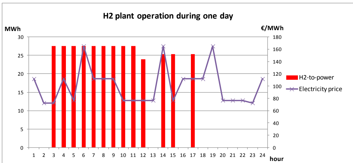
Fig.7 - Power supply from hydrogen fuel cell as a function of the market price
