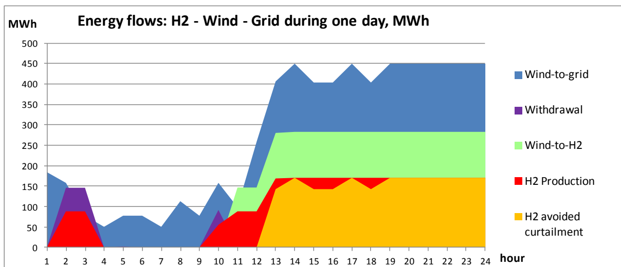
Fig. 5 - Wind and hydrogen energy flows during one day
