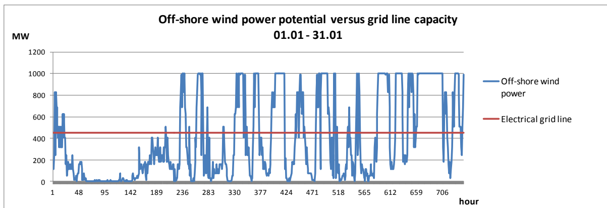
Fig. 3 - Representation of the potential wind power and the grid transmission line during one month
