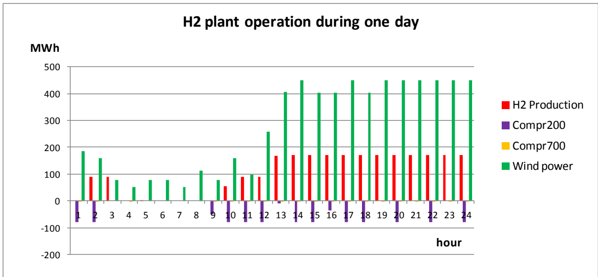
Fig. 6 - The operation of the hydrogen plant during one day
