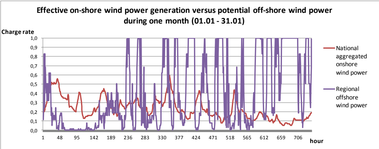
Fig. 2 - Fluctuation of effective on-shore wind power and potential off-shore wind power
