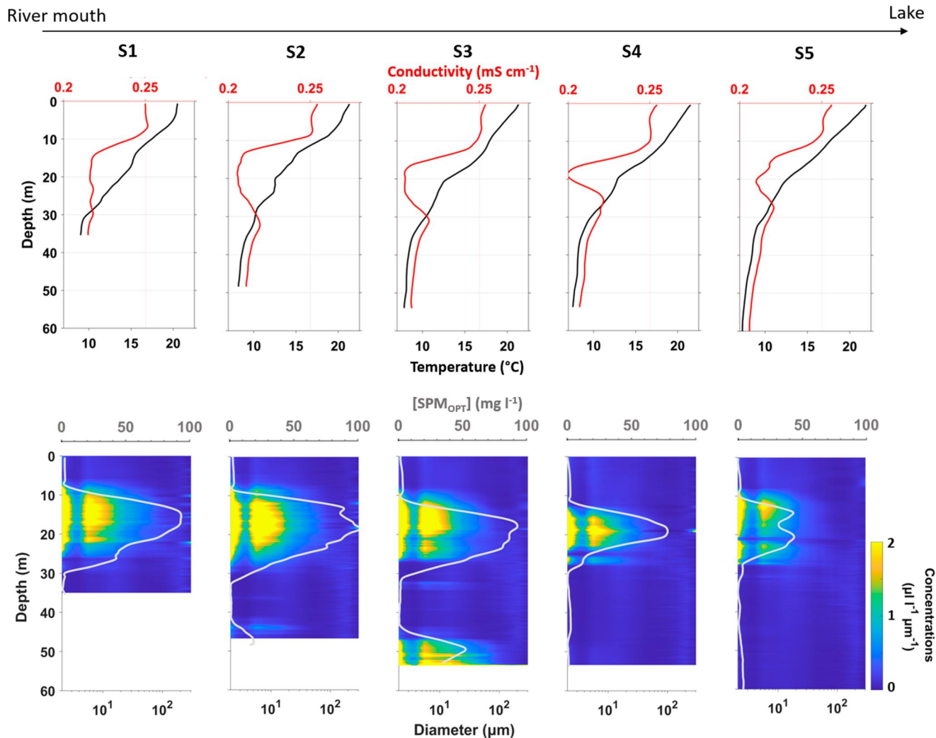
Figure 3. For the five stations S1–S5 along the interflow plume. Top panels: profiles of temperature (black lines) and electrical conductivity at 25°C (red lines). Bottom panels: SPM OPT profiles (gray lines) plotted over concentration profiles of particles per size class (color maps, from LISST-100X). The colorbar gives the (volume) particle concentration per size class ( \mu\text{l l}^{-1} \mu\text{m}^{-1} ). At each station, profiles are shown to the lake bed. For station locations, see Figure 1b.
