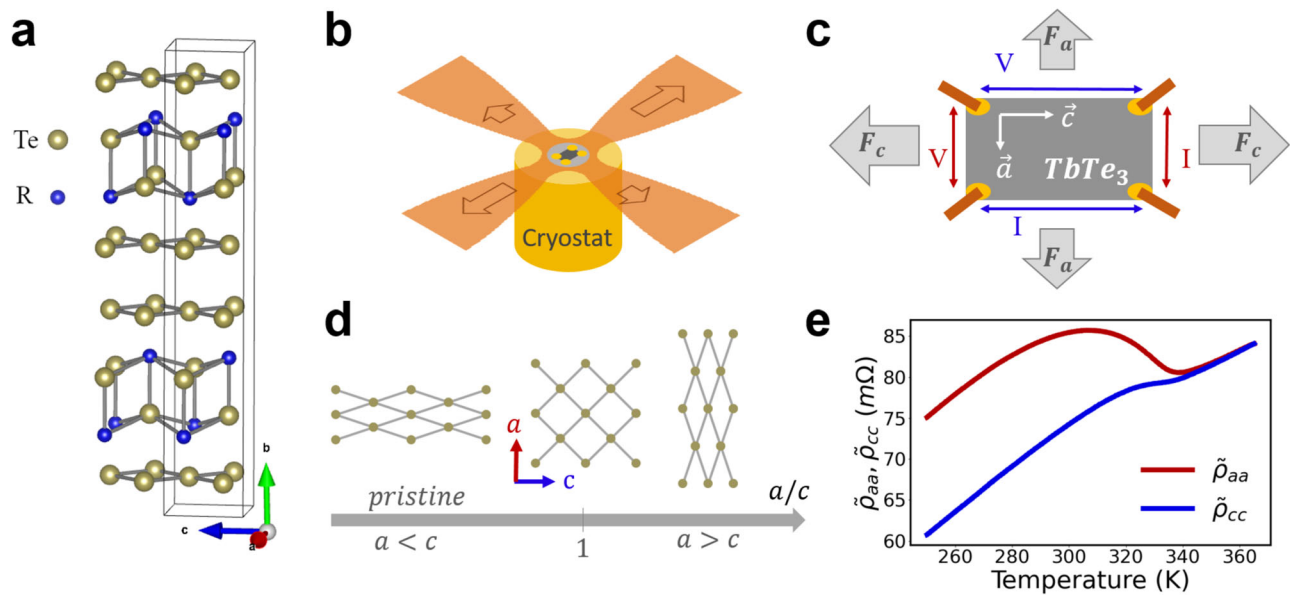
Fig. 1 | Principle of cryogenic biaxial deformation of TbTe_3 . a The RTe_3 crystal structure is quasi-tetragonal (unit cell shown in black), and made of a succession of RTe slab intercalated by two quasi-square Te planes in the (a, c) planes. The two in-plane directions are non-equivalent due to the presence of a glide plane along c (space group Cmcm ) which leads to a slight orthorhombicity ( 1 - \frac{c}{a} \sim 1.3 \cdot 10^{-3} in TbTe_3 at 300 K 10 ). b Schematic drawing of the biaxial tensile stress device: a thin crystalline sample is glued on a polyimide cross-shaped substrate on which tensile stresses are applied along the arms. The main in-plane directions of the crystal a and c are aligned with the arms of the cross. The bottom side of the cross is in contact with the cold finger of a nitrogen-flow cryostat. c Four electrical contacts
