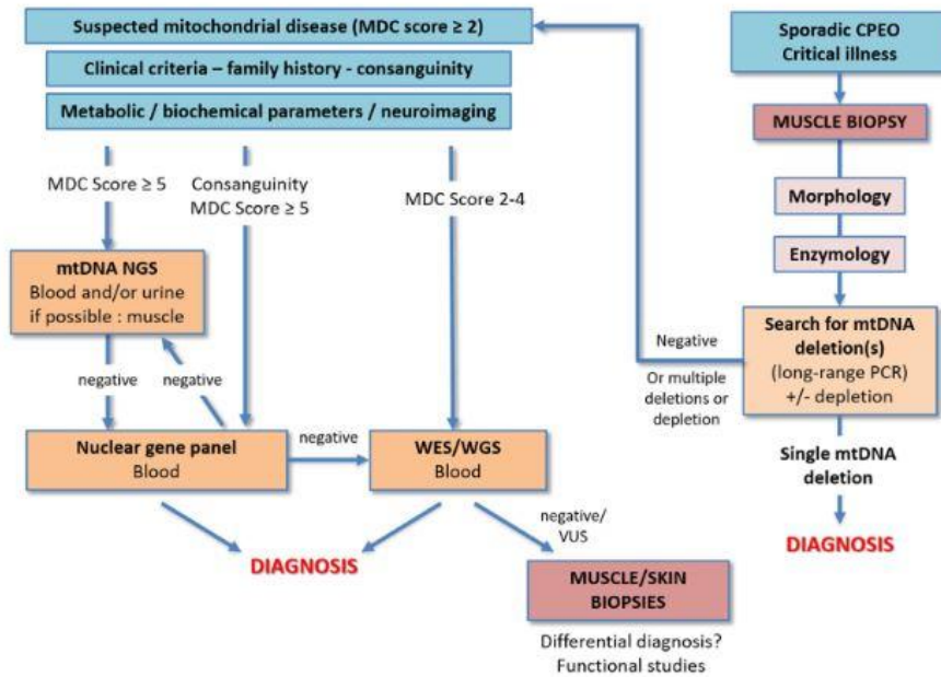
Figure 5. Diagnostic approach for mitochondrial disorders. Score 2-4: possible PMD, score \geq 5 probable PMD.
