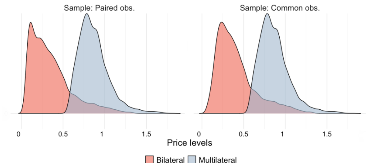
Figure 1 — Distributions of bilateral and multilateral real exchange rates in levels
