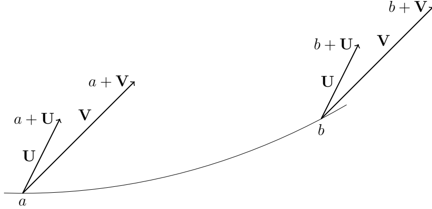
Fig 3 : Discrepancy in size measurement a hold a stick (a, a + U) and b a stick (b, b + V) . exchanging their measurement of length a and b may find d_a(a, a + U) = d_b(b, b + V) while a alone finds d_a(a, a + U) \neq d_a(b, b + V)
