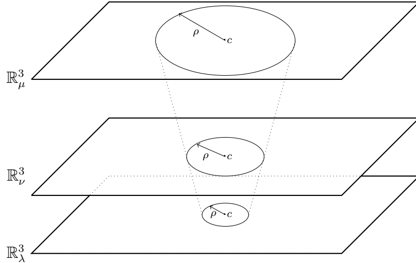
Fig 2 : Circles with same radii and centers in \mathbb{R}_\mu^3, \mathbb{R}_\nu^3 and \mathbb{R}_\lambda^3 with \lambda > \mu > \nu
