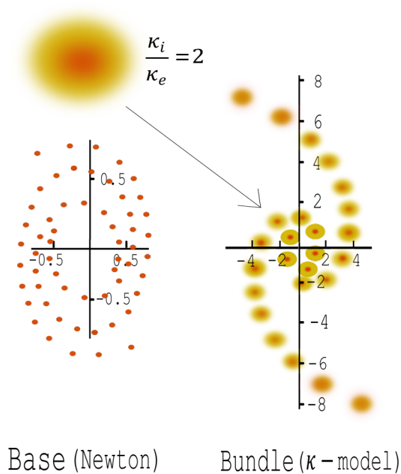
Fig 9 : A toy example : A well-developed conservative spiral substructure seen in the bundle as opposed to its counterpart living in the base (a tightly coiled spiral)
