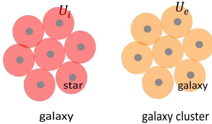
Fig 13 : Stacking of balls covering a galaxy or a galaxy cluster
