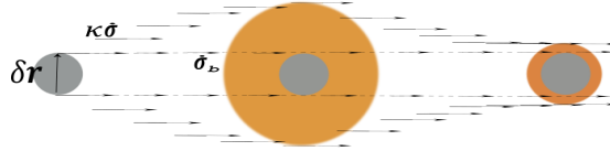
Fig 15 : Apparent variation of a disk of constant size seen from the point of view of a terrestrial observer. The real size is the disk shown in gray.
