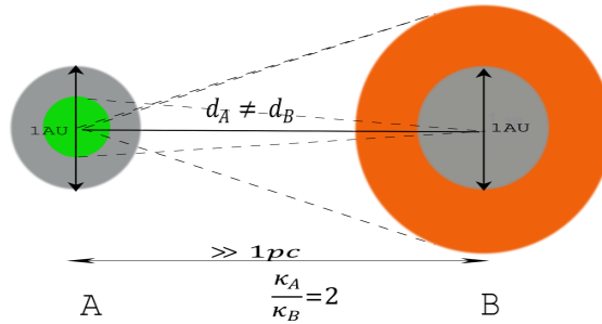
Fig 4 : Discrepancy in size measurement for a disk
