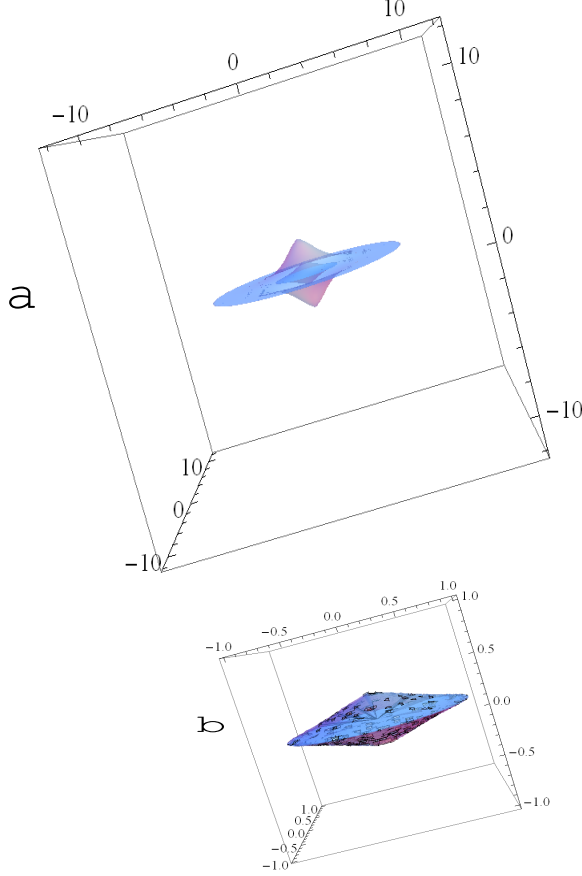
Fig 11 : A side-on galaxy seen by a terrestrial observer (a) as opposed to its compact counterpart living in the base (b). On this illustrative example the terrestrial observer measures the density \rho(r, z) = \exp(-r - (5 + r)|z|) .
