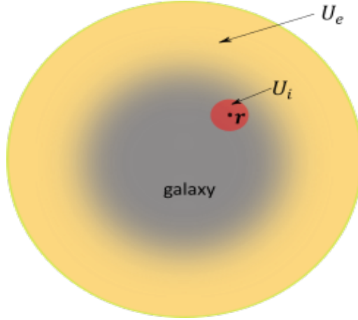
Fig 12 : Averaging over a ball surrounding a star or a galaxy
