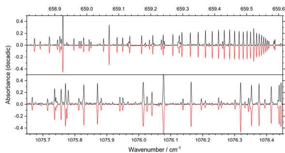
Fig. 31. Top panel: Experimental (upward) and simulated (downward) spectra of HCOOH within the \nu_9 fundamental using a Gaussian FWHM of 0.00171 cm -1 . Bottom panel: Experimental (upward) and simulated (downward) spectra spectra within the \nu_6 fundamental using a Gaussian FWHM of 0.00245 cm -1 .
