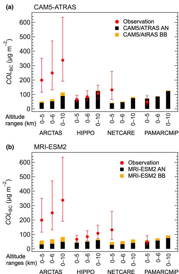
Figure D2. Observed column amounts of BC mass concentration for 0–5, 0–6, and 0–10 km altitude ranges at latitudes >66.5^\circ N ( COL_{BC} , red circles) and model-calculated COL_{BC} values (vertical bars). For calculated values, contributions from anthropogenic (AN) and biomass burning (BB) emissions are shown by black and orange colors, respectively. The model-calculated COL_{BC} values were derived by calculating area-weighted averages within the areas and time periods of the individual aircraft-based experiments. (a) CAM5-ATRAS model simulations. (b) MRI-ESM2 model simulations.
