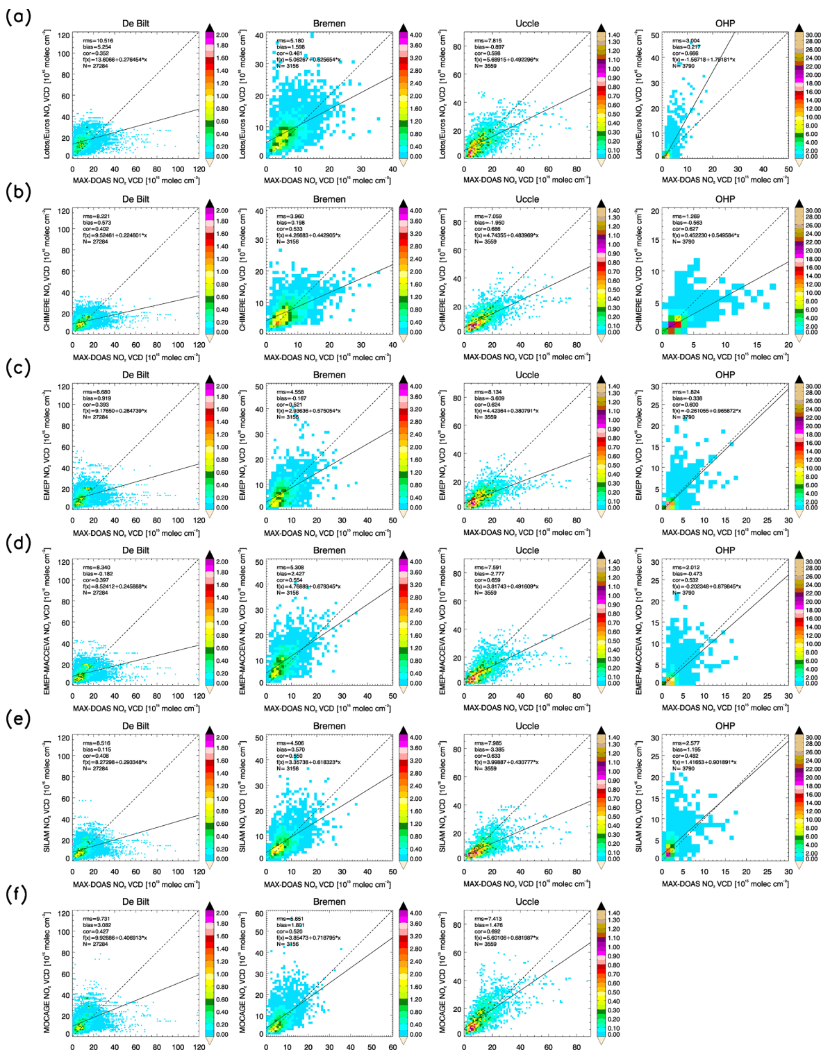
Figure A2. Scatter density plots of AVK-weighted tropospheric NO 2 VCDs ( 10^{15} molec cm -2 ) from MAX-DOAS against model data for (from left to right) De Bilt, Bremen, Uccle and OHP. The data are shown for different bins with a size of 10^{15} molec cm -2 and are colored according to the number of data points per bin (%). The different panels show different model runs: (a) LOTOS-EUROS, (b) CHIMERE, (c) EMEP, (d) EMEP-MACCEVA, (e) SILAM and (f) MOCAGE. MOCAGE data are not available for the measurement time period at OHP. The dashed line is the reference line ( f(x) = x ). The solid line is the regression line (see top left of each plot for f(x) of this line). The root mean squared error (RMSE) ( 10^{15} molec cm -2 ), bias ( 10^{15} molec cm -2 ), Pearson correlation coefficient (cor, not squared) as well as the number of data points N are given in the top left of each plot.
