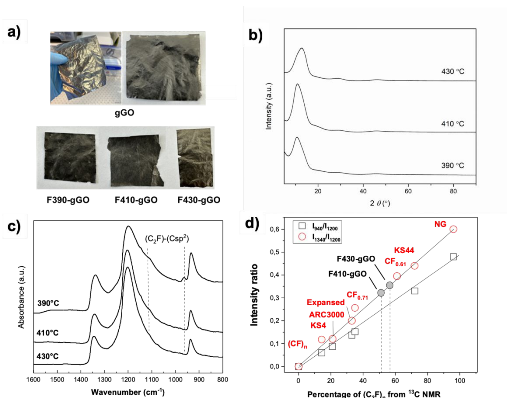
Figure 5. Photographs of gGO foils before and after fluorination (a). XRD patterns of fluorinated gGO foils (b). IR spectra of the fluorinated gGO films. The intensity ratio of the lines typical of (C_2F)_n phase as
