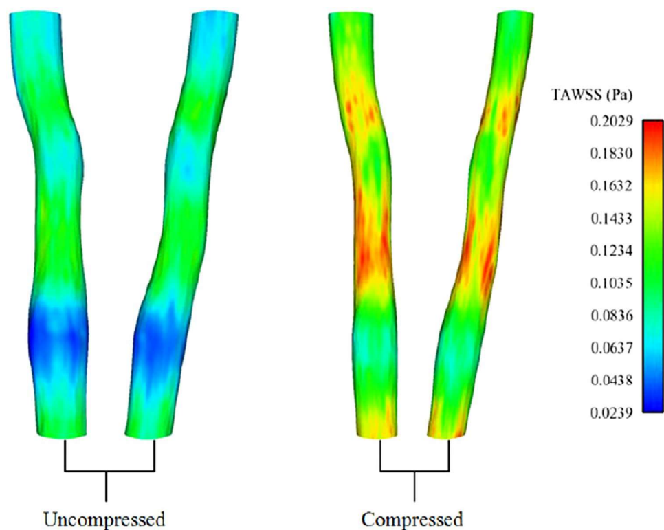
Fig. 6 Representative time-averaged wall shear stress maps in the peroneal vein obtained from MRI-based CFD simulations before (left) and after (right) compression. Extracted with permission from Wang et al. [181]
