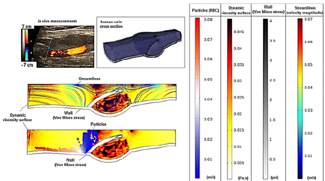
Fig. 5 Use of in vivo flow visualization to validate FSI modeling. Top left: in vivo Doppler ultrasound images and mesh reconstruction of venous valve geometry. Bottom left: FSI simulation of leaflet stress and surrounding fluid flow during valve opening. Right: Extracted
