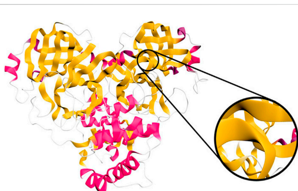
FIGURE 12 Narupa iMD rendering of the ribbon representation of the SARS-CoV-2 main protease (PDB ID: 6W63). Image by under a CC-BY DEED 4.0 licence, reproduced from (Jamieson-Binnie and Glowacki, 2021).
