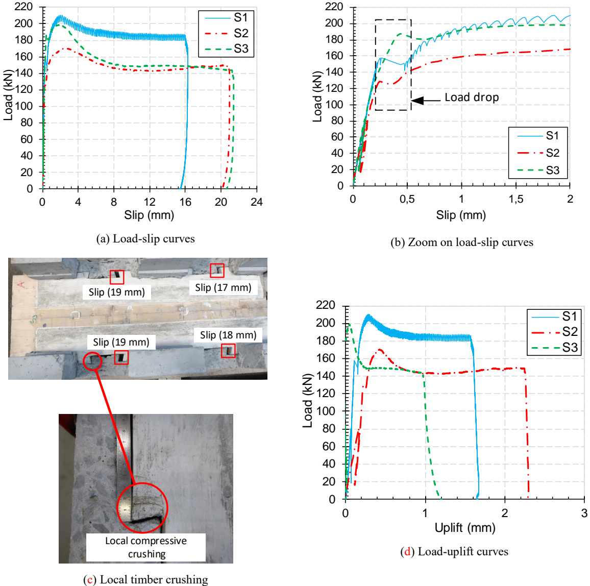
Figure 4: Force-slip and force-uplift curves of the push-out tests.
