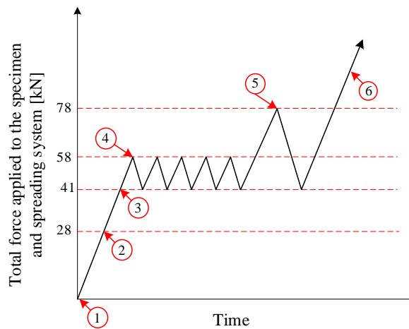
Figure 13: Loading procedure for test F1.
