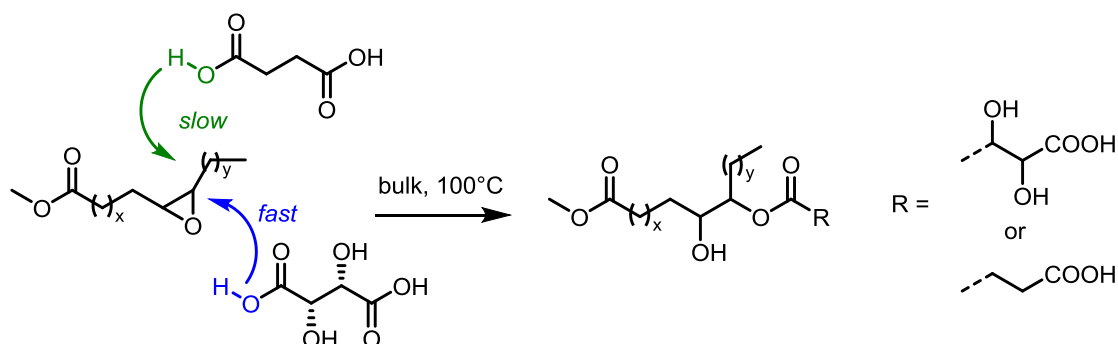
Figure 3- Molecular model reaction used to compare tartaric and succinic acid with epoxidized methyl oleate, reaction conditions: bulk, 100°C, up to 24h, [\text{COOH}] = 2 [EMO].
