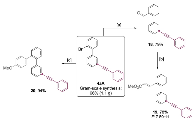
Scheme 5. Post-functionalization reactions of the meta -alkynylated product 4aA . [a] n BuLi (2 eq.), DMF (10 eq.), THF, -78^{\circ}\text{C} to RT, 2.5 h; [b] methyl (triphenylphosphoranylidene)acetate (1.5 eq.), DCM, RT, 48 h; [c] Pd(PPh 3 ) 4 (3 mol %), K 2 CO 3 (10 eq.), 4-CH 3 O-C 6 H 4 B(OH) 2 (4 eq.), Toluene/H 2 O/EtOH 4:1:1, 120 ^{\circ}\text{C} , overnight.
