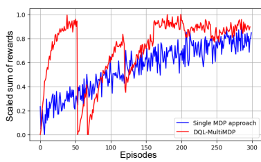
Fig. 3: MDP decomposition
