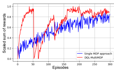
Fig. 3: MDP decomposition
