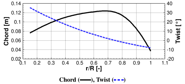
Fig. 2 Chord and twist distributions of HAD-1 blade.
