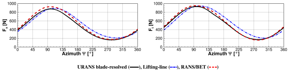
Fig. 29 Blade axial and tangential loads over a revolution (9° incidence angle).
