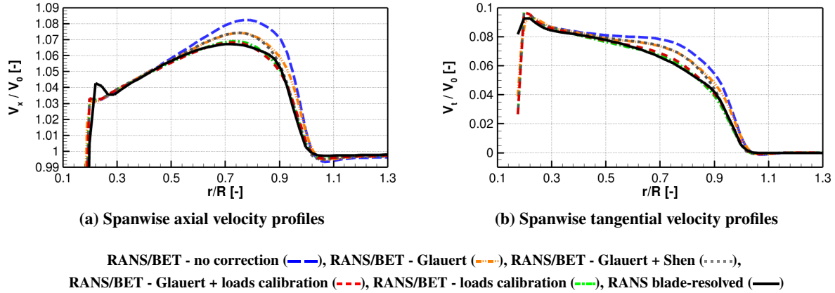
Fig. 23 Wake velocity profiles for each tip-loss correction.
