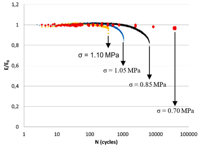
Fig. 23. Relative modulus evolution under different loading amplitudes.
