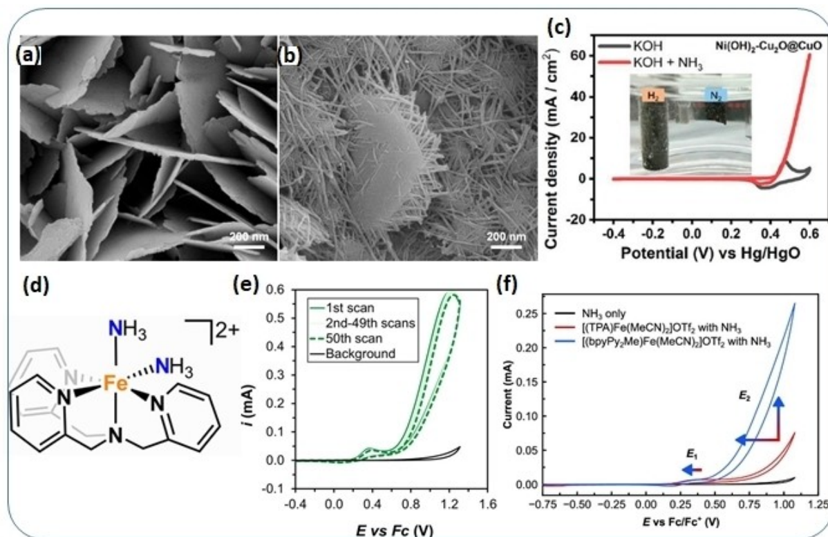
Figure 7. SEM images of (a) \text{Ni}(\text{OH})_2 nanoplates and (b) \text{Ni}(\text{OH})_2\text{-Cu}_2\text{O}@/\text{CuO} wire-on-plates. (c) Voltammograms of \text{Ni}(\text{OH})_2\text{-Cu}_2\text{O}@/\text{CuO} electrode recorded in 1 M KOH and 1 M KOH + 1 M \text{NH}_3 . Reproduced with permission. [72] Copyright 2020 ACS. (d) Chemical structure of [(\text{TPA})\text{Fe}(\text{NH}_3)_2]\text{OTf}_2 and (e) CV recorded with boron doped diamond electrode in 2.5 mM [(\text{TPA})\text{Fe}(\text{MeCN})_2]\text{OTf}_2 in acetonitrile solution containing 50 mM \text{NH}_3 and 50 mM \text{NH}_4\text{OTf} . Reproduced with permission. [74] Copyright 2019 ACS. (f) Voltammograms of boron doped diamond electrode in acetonitrile containing 0.2 M \text{NH}_3 only (black) and with 0.5 mM [(\text{TPA})\text{Fe}(\text{MeCN})_2]\text{OTf}_2 (red) and [(\text{bpyPy}_2\text{Me})\text{Fe}(\text{MeCN})_2]\text{OTf}_2 . Reproduced with permission. [75] Copyright 2021 ACS.
