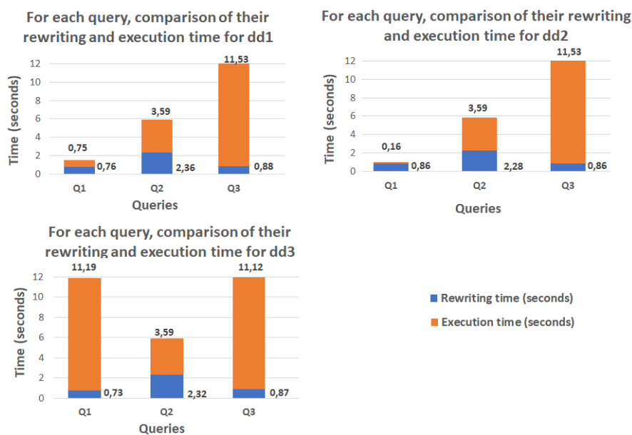
Fig. 5. Experiment result for query rewriting time and query execution time for the three polystore distribution considered in this paper considering the execution over the relational unified model
