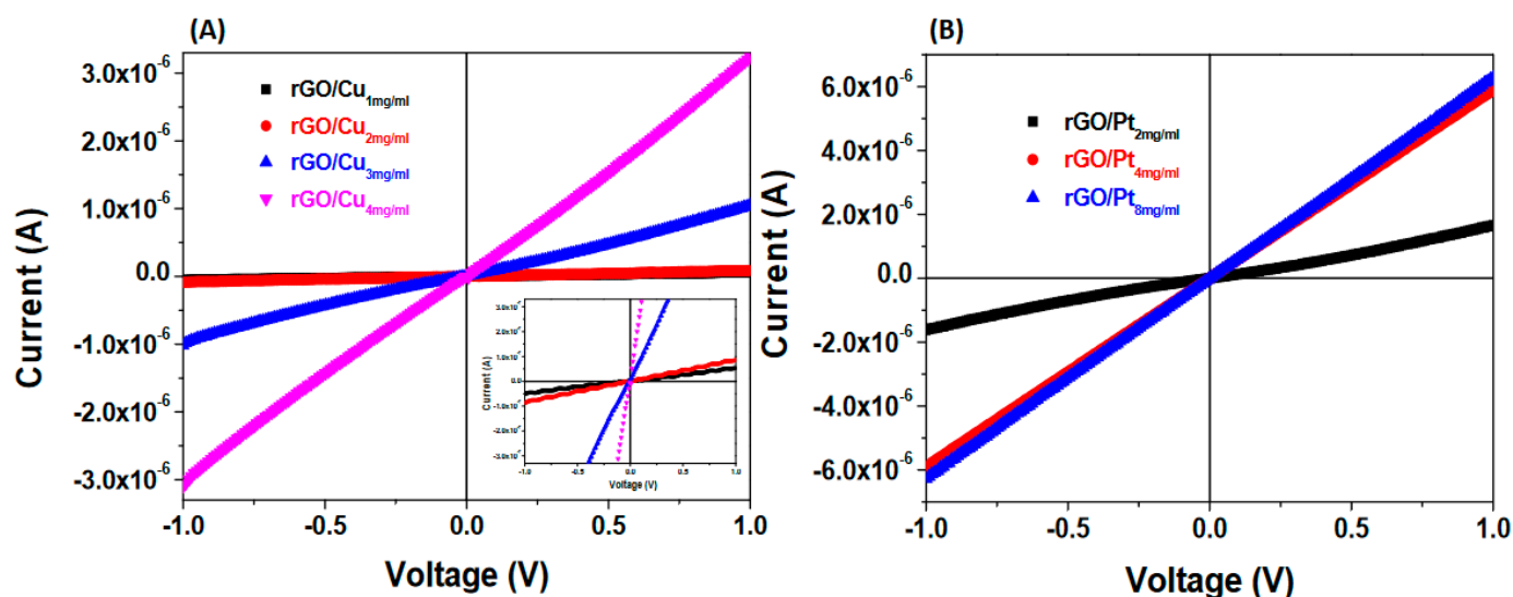
Figure 4. Current-voltage characteristics of rGO/Cu (A) and rGO/Pt (B) nanocomposites obtained by chemical decoration. The inset in Figure 4A shows a zoom on the y axis to highlight the overlapping curves (the red and black curves).
