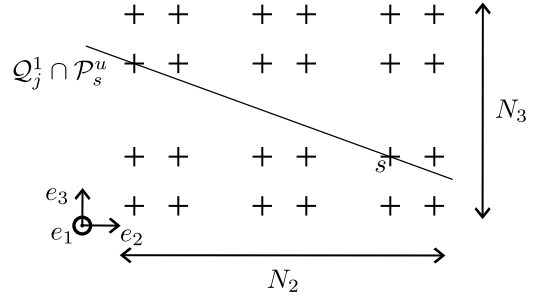
Fig. 7. Intersection of \mathcal{Q}_j^1 and \mathcal{P}_s^u when \mathbf{u} and \mathbf{e}_1 are not orthogonal
