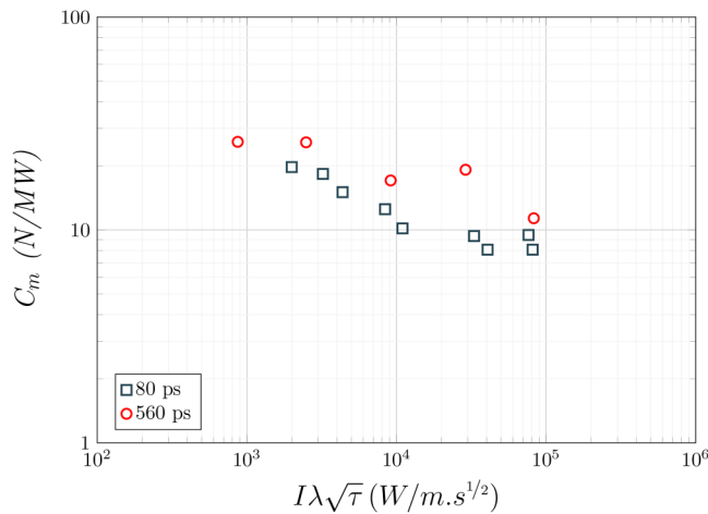
FIG. 8. Pulse duration influence on the momentum coupling. Shots from ELFIE2018 campaign for 560 and 80 ps pulses, spot sizes are, respectively, 4.6 and 5.5 mm.
