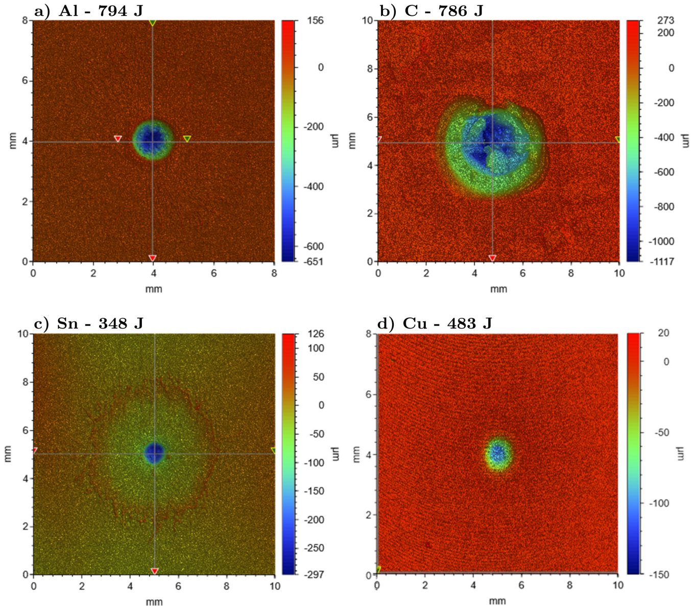
FIG. 13. Profilmeter imaging of the crater for (a) aluminum, (b) carbon, (c) tin, and (d) copper for shots of the LULI2020 and LULI2021 campaigns.
