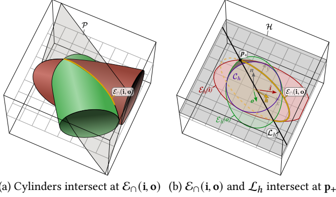
Fig. 19. Geometry of the shadow overlap region. (a) The cylinders oriented along \mathbf{i} and \mathbf{o} (in red and green respectively) and tangent to the unit spherical micrograin (not shown) intersect in an ellipse \mathcal{E}_n(\mathbf{i}, \mathbf{o}) , which lies in a plane \mathcal{P} . (b) We then compute several intersections with the plane \mathcal{H} at height h : with \mathcal{P} to get the line \mathcal{L}_h , with the unit sphere to get \mathcal{C}_h , and with the cylinders from (a) to get \mathcal{E}_h(\mathbf{i}) and \mathcal{E}_h(\mathbf{o}) . The shadow overlap region (in gray) is then found by using points where \mathcal{E}_h(\mathbf{i}) and \mathcal{E}_h(\mathbf{o}) are tangent to \mathcal{C}_h , and the point \mathbf{p}_+ at the intersection of \mathcal{L}_h and \mathcal{E}_n(\mathbf{i}, \mathbf{o}) .
