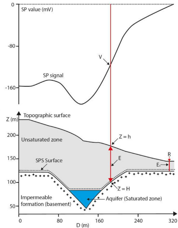
Fig. 2. Some examples of SP profile in the context of the Chaîne des Puy. (A) Typical case of an SP signal in the context of a paleo-valley filled with volcanic formations and a flat topography. (B) Representation of a SP signal in a particular context with the different numerical parameters entering in the SPS modeling [1,3].
