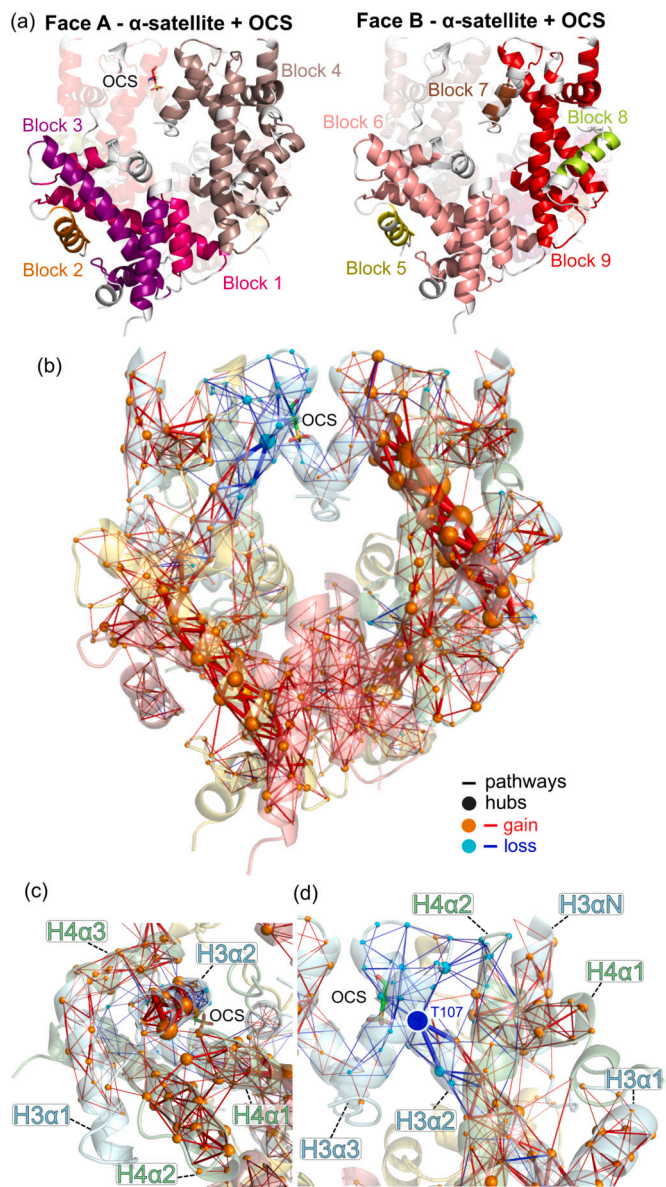
Fig. 5. (a) Communications blocks in the \alpha -satellite NCP with cysteine S-sulfonylation (OCS), on face A and face B. (b) Perturbation of communication pathways upon S-sulfonylation, viewed from face B. Red paths/hubs are gains with the modification, blue are losses. (c) Bottom view of H3' \alpha 2 helix (in communication Block 4), through which multiple pathways connect other H3' and H4' helices. (d) Weakened pathways around the S-sulfonylated cysteine. T107 is highlighted by a white-blue circle.
