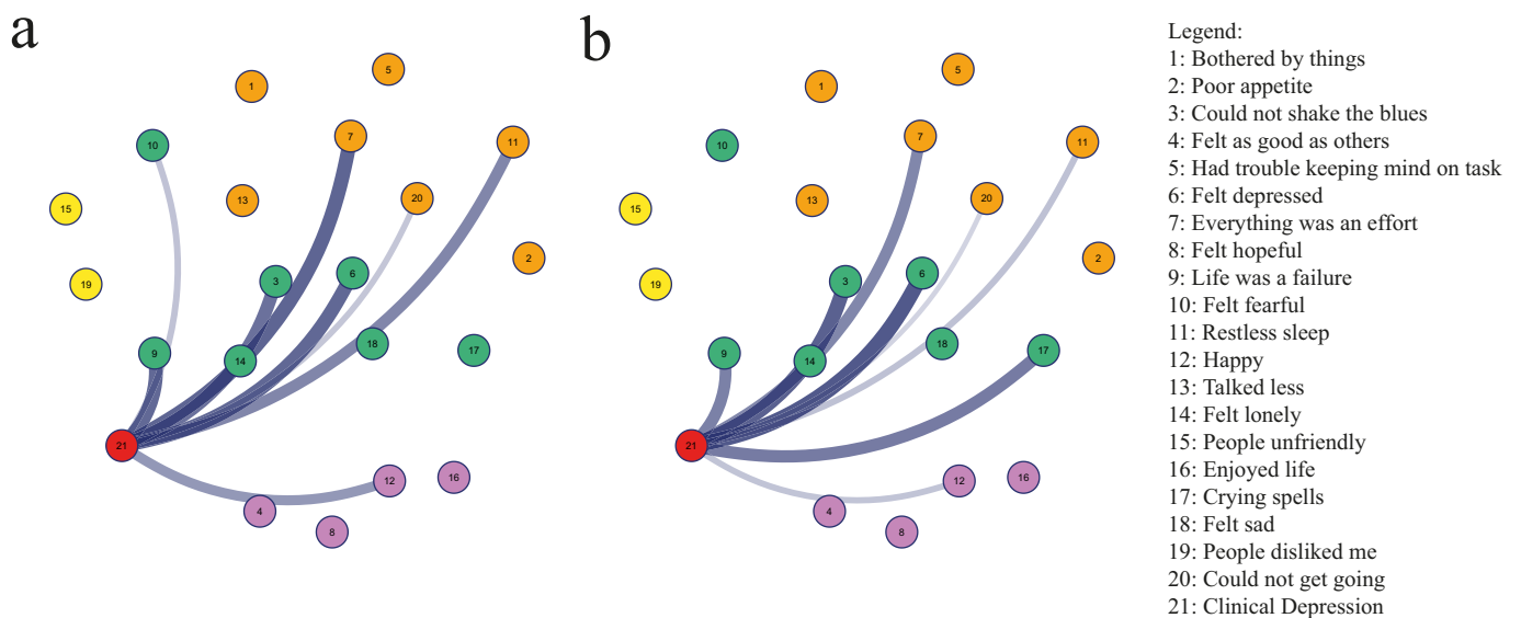
Fig. 3. Connections between depressive symptoms and Clinical Depression as an external factor (node 21). Panel ‘a’: women ( n=108,391 ). Panel ‘b’: men ( n=93,561 ). Edges’ widths were scaled to the closest higher value than any absolute edge weight in order to facilitate comparisons across sexes. Edges were curved to avoid overlapping. Items were colored by dimensions (factors); Green: depressive affect, Purple: positive affect; Orange: somatic; Yellow: interpersonal.
