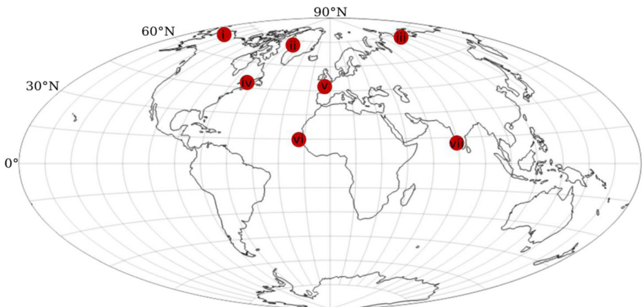
Fig. 1 Location of the study sites: (i) Wainwright (Alaska, USA), (ii) Uummanaq (Greenland), (iii) Tiksi (Sakha (Yakutia) Republic, Russian Federation), (iv) Cocagne-Grande-Digue (New Brunswick, Canada), (v) Bay of Brest (Brittany, France), (vi) Mbour (Senegal), (vii) Vypin Island-Chellanam Peninsula (Kerala state, India)
