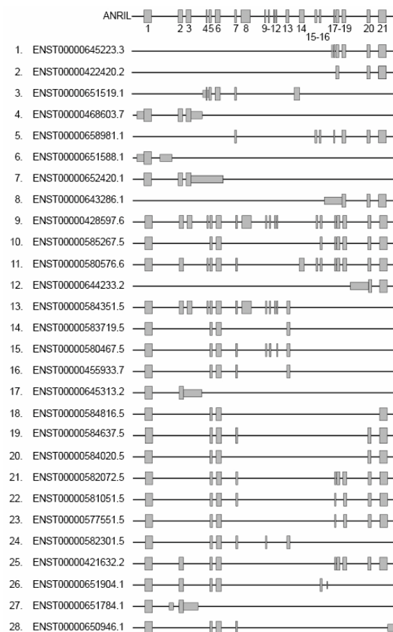
Figure 2. Representation of the different linear isoforms of ANRIL. Grey rectangles represent exons, numbered from 1 to 21. The left side displays isoform accession numbers from the Ensembl database along with alternative nomenclature ranging from 1 to 28.
