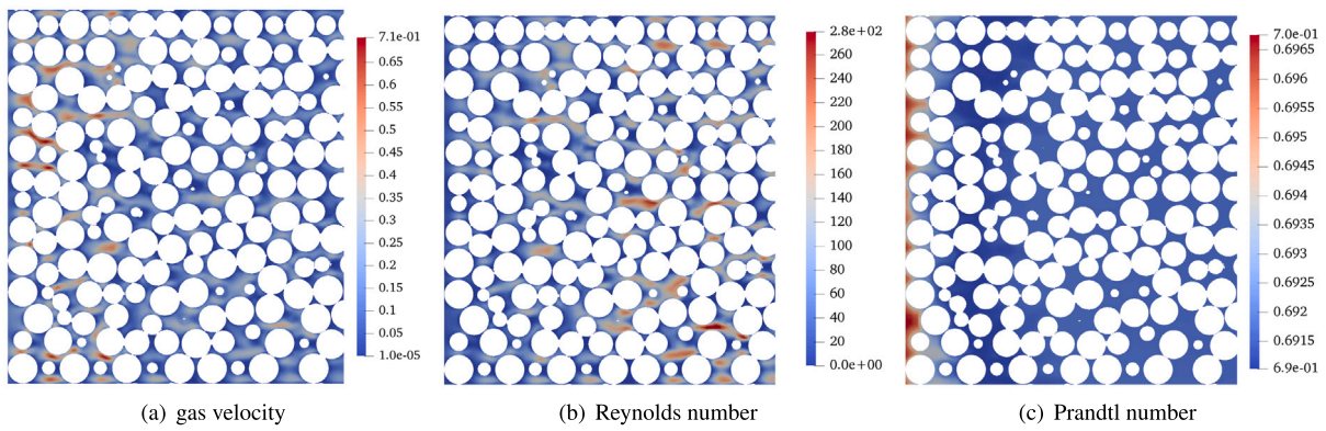
Fig. 12. Gas velocity, Reynolds number, and Prandtl number distribution in Section 1 of the randomly packed bed with an inlet velocity of 0.1 m/s and a time of 1000 s.
