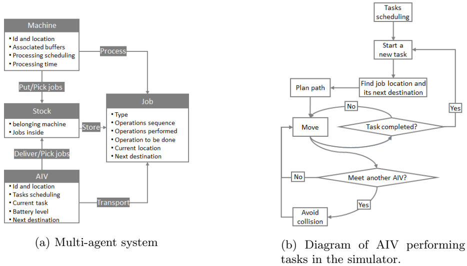
Fig. 2: Simulation framework
