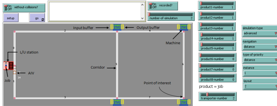
Fig. 3: Simulation interface
