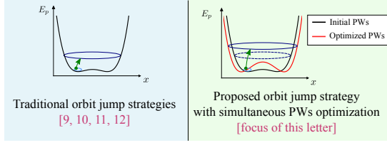
FIG. 1. Comparison of the proposed approach with traditional orbit jump strategies. The dashed high orbit corresponds to the high orbit obtained with a traditional orbit jump strategy, i.e., without PWs optimization.
