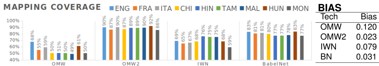
Figure 2: Bias in the expressivity of cross-lingual mappings of multilingual lexical databases. Left: per-language coverage (performance) of mappings for each database. Right: bias of each database.
