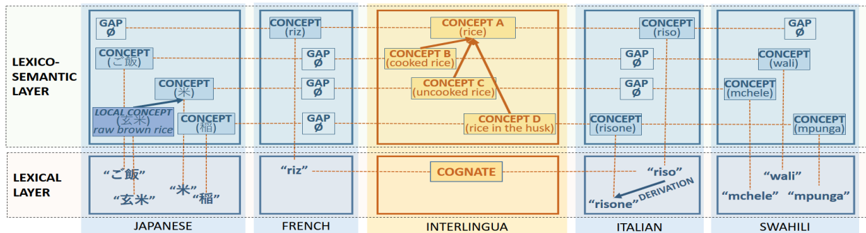
Figure 3: The cross-lingual mapping model of the UKC lexical database.
