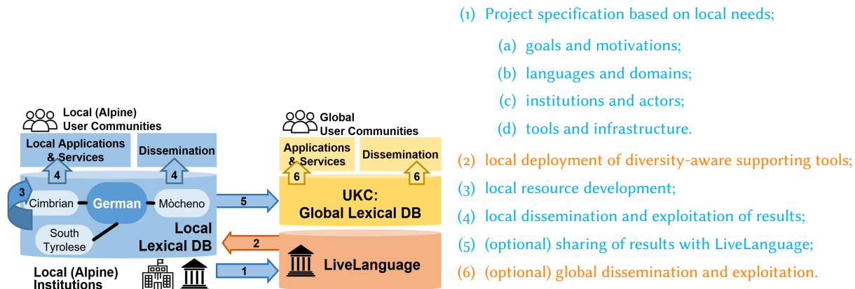
Figure 4: Collaborative language development methodology in the framework of the LiveLanguage initiative
